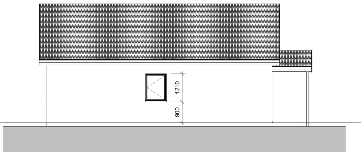
2 Elevation 2 - North 1 : 100
