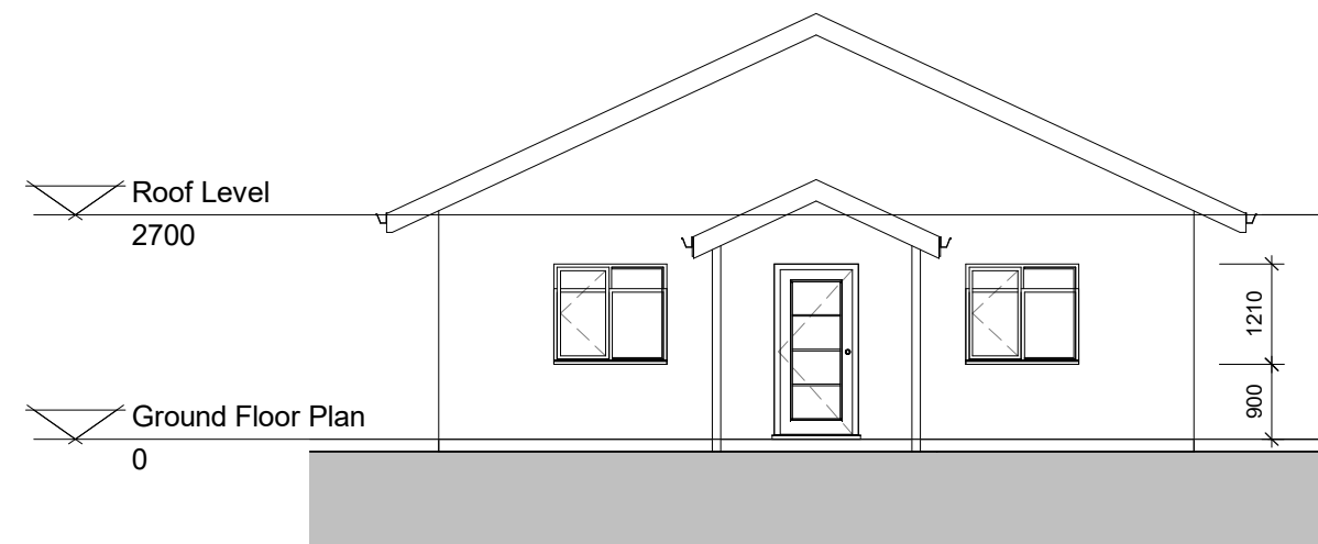
1 Elevation 1 - West 1 : 100
