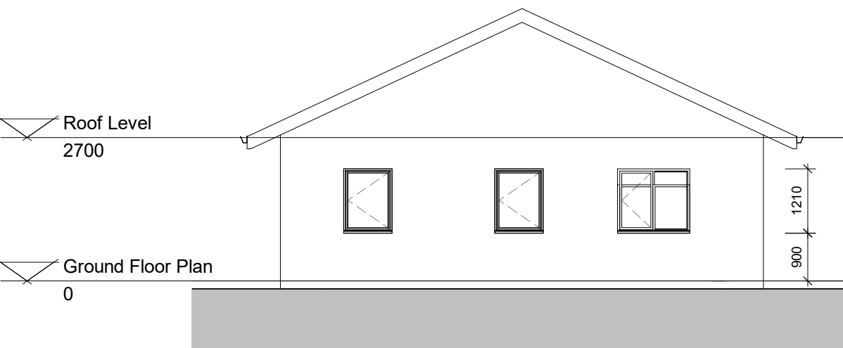
3 Elevation 3 - East 1 : 100
