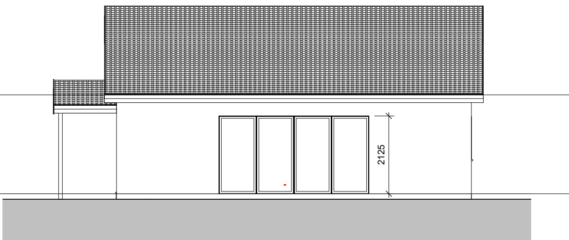
4 Elevation 4 - South 1 : 100
