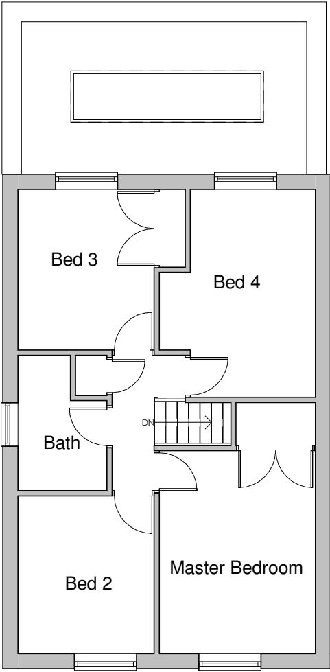
First Floor 1 : 100
