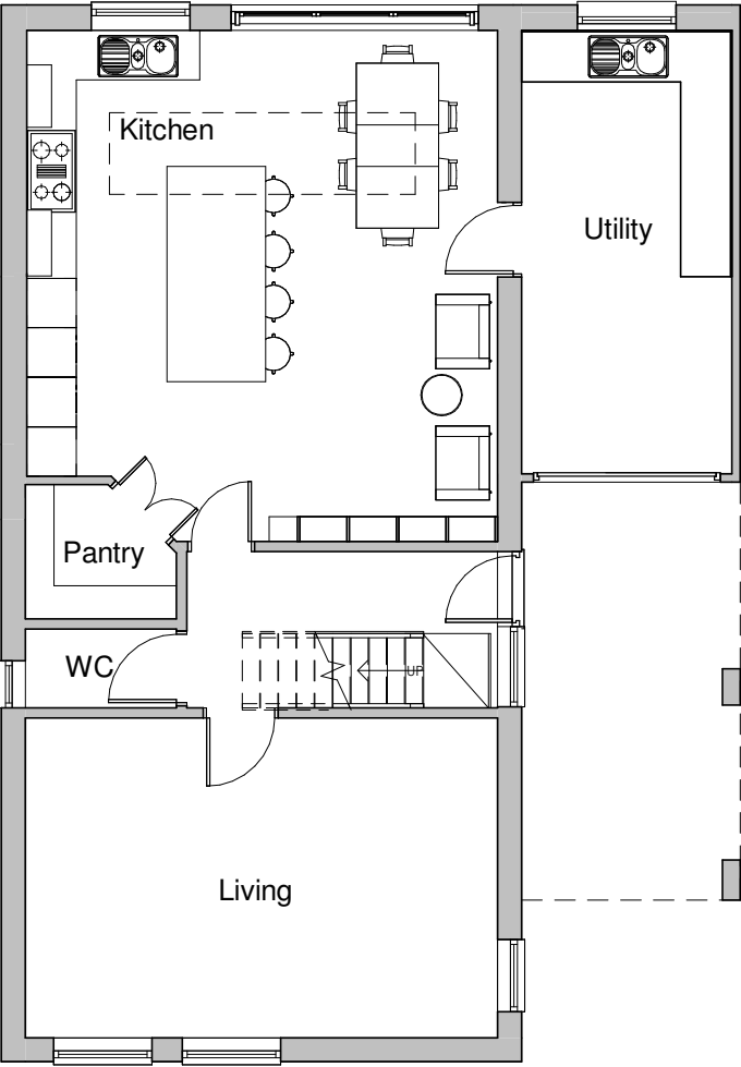
Ground Floor 1 : 100
