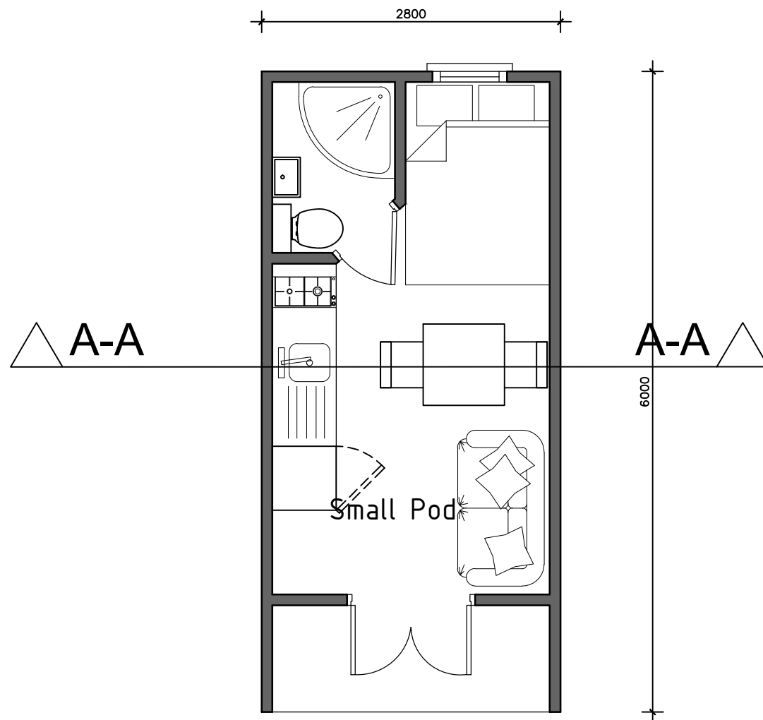
Ground floor plan 1:50
