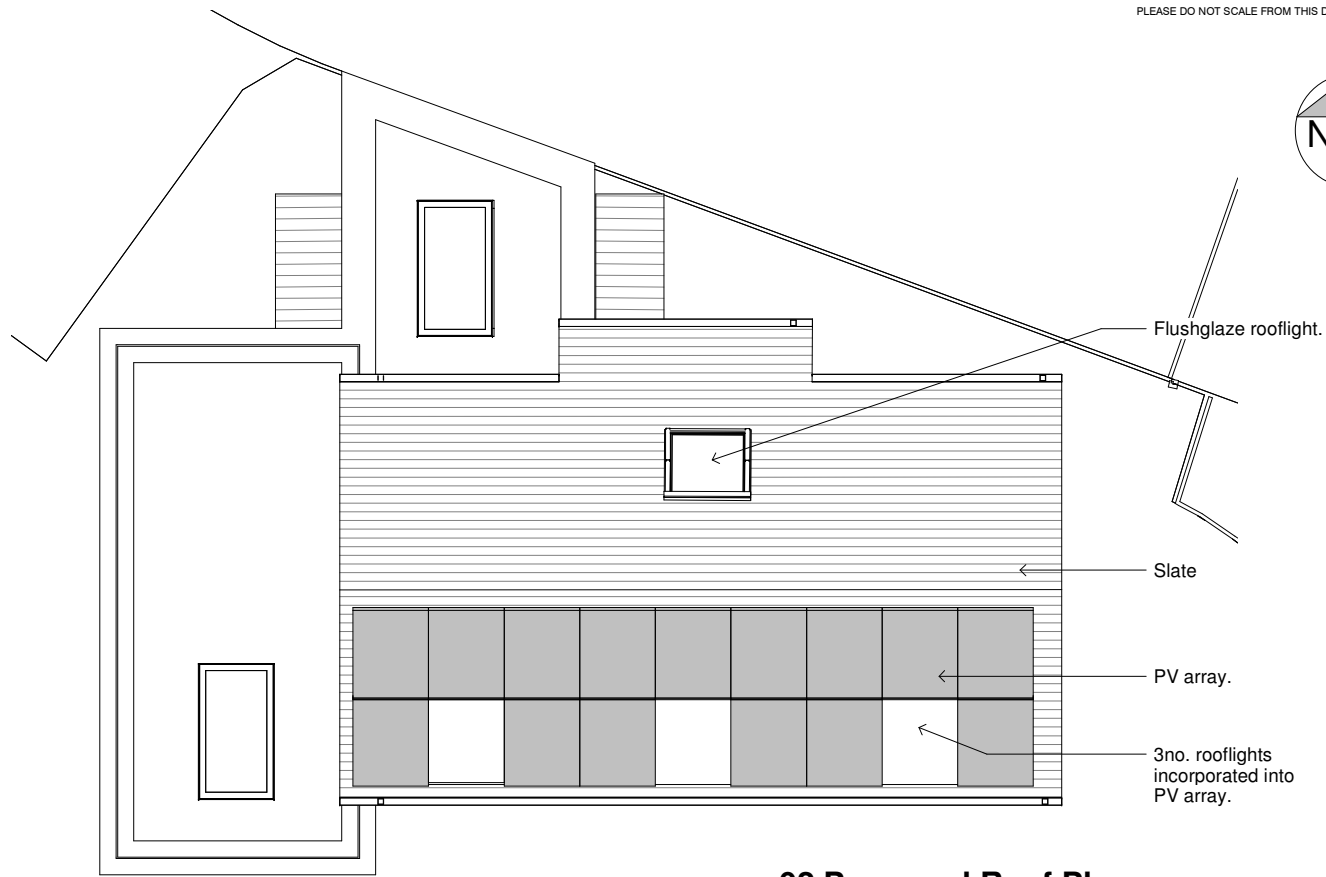
02 Proposed Roof Plan 1 : 50 (1 : 100 @ A3)
