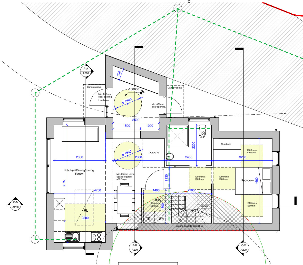
00 Proposed Ground Floor 1 : 50 (1 : 100 @ A3)
