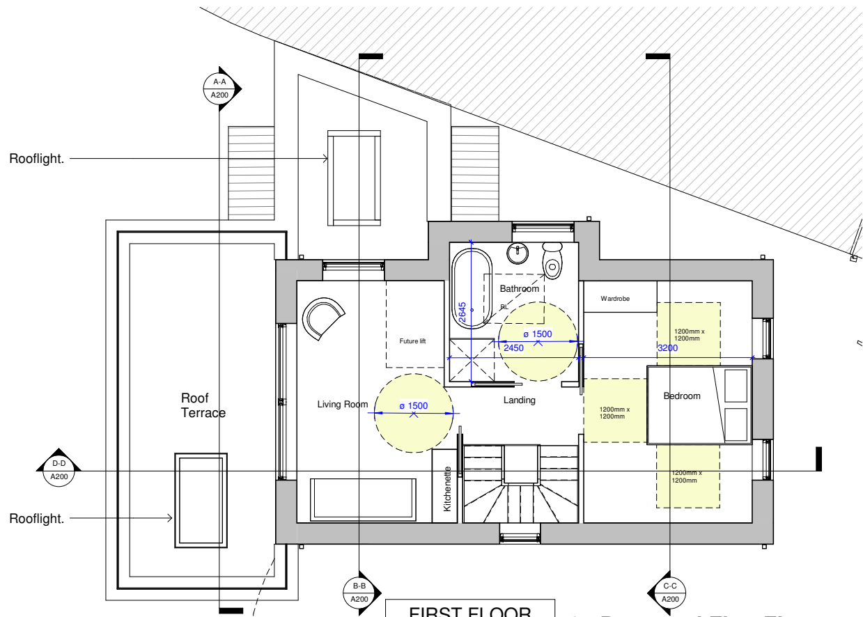
01 Proposed First Floor 1 : 50 (1 : 100 @ A3)
