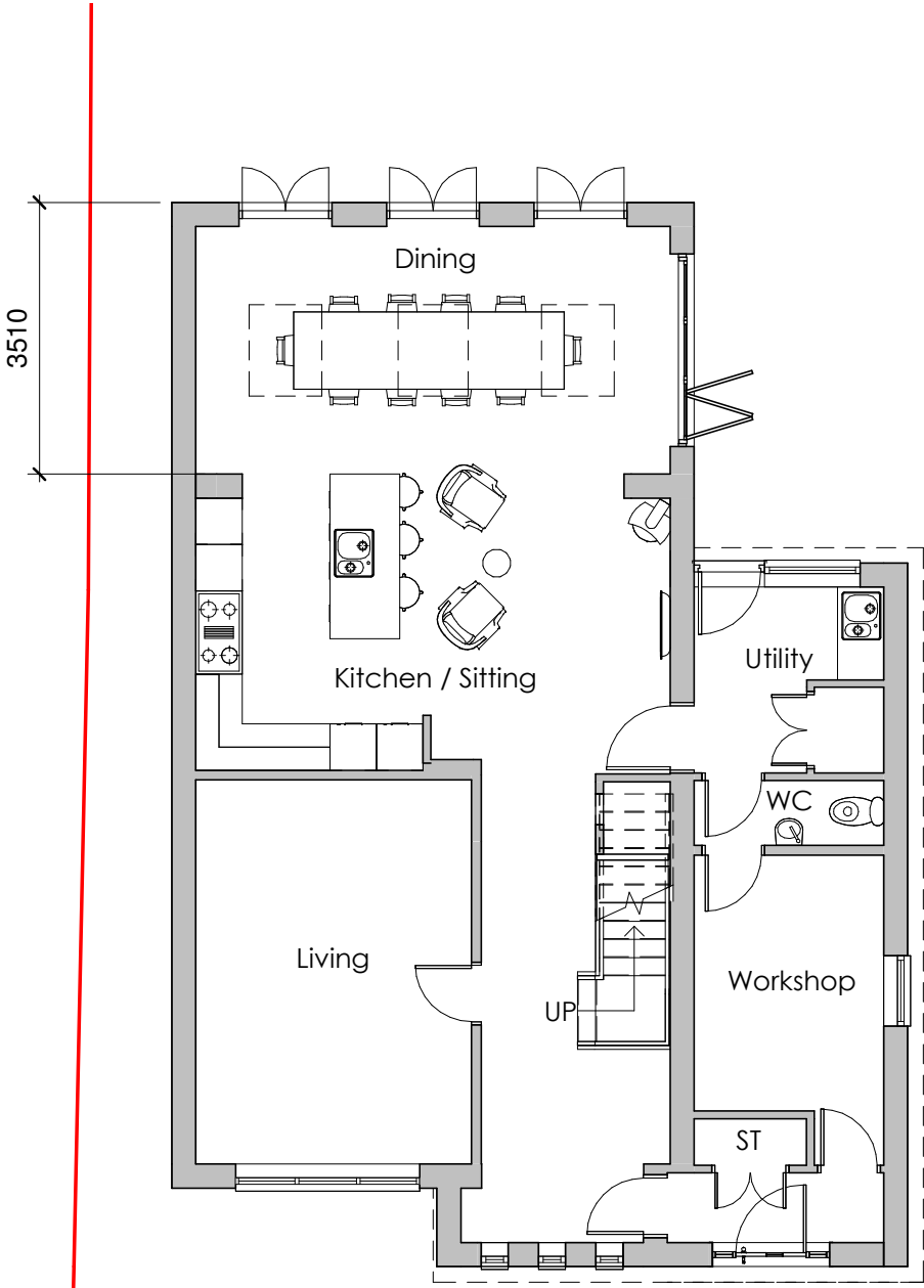
Ground Floor 1 : 100
