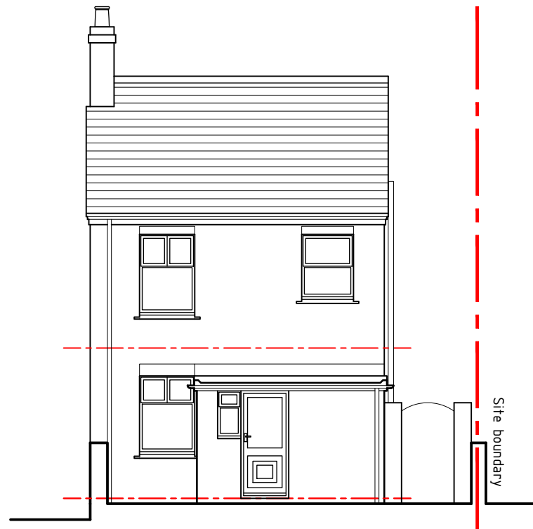
Rear Elevation 1:100
