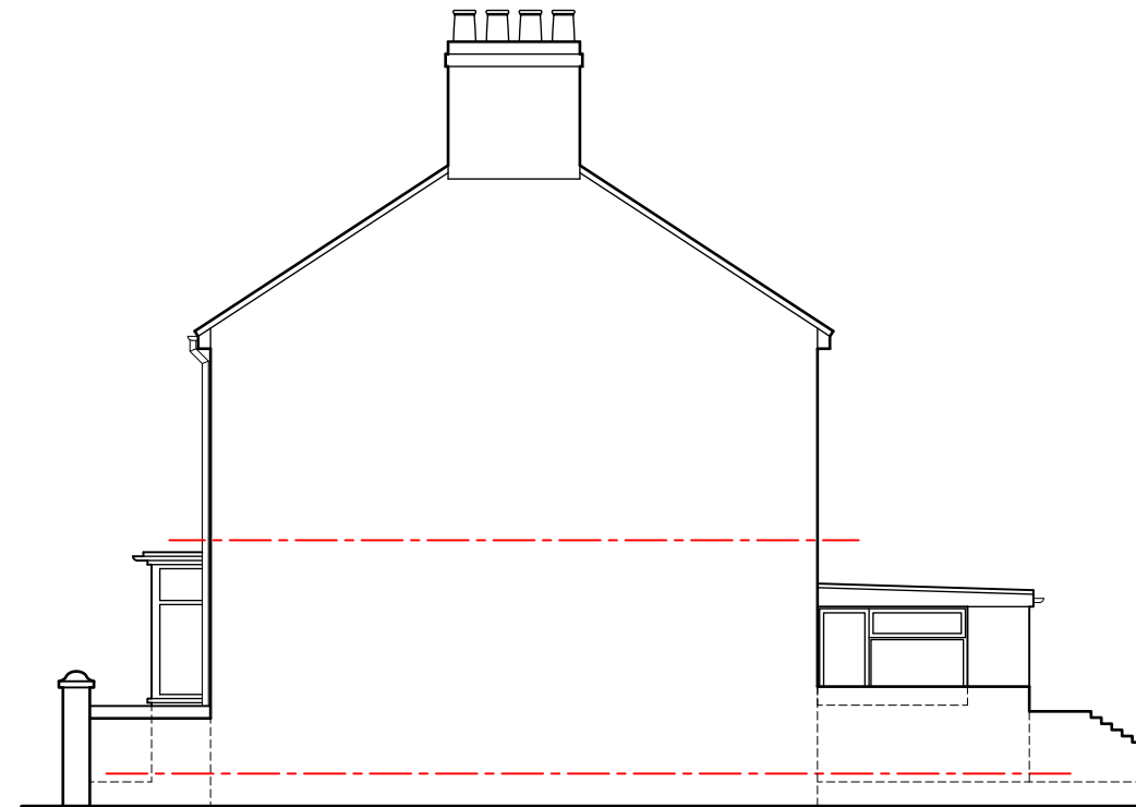
Side-2 Elevation 1:100
