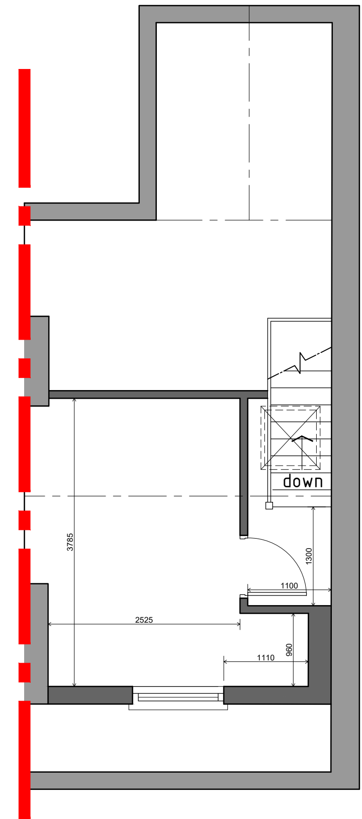
ATTIC
