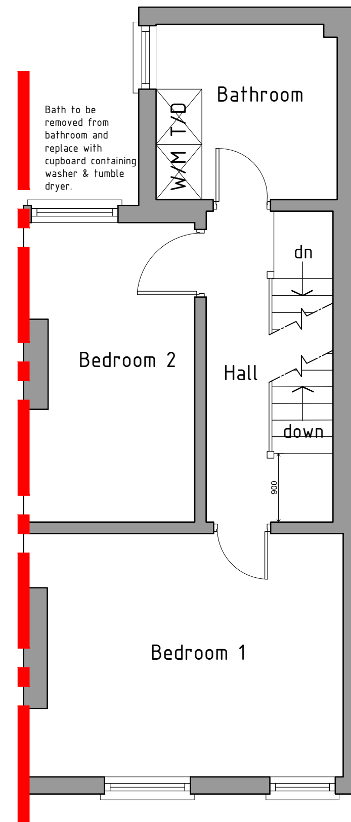
FIRST FLOOR
