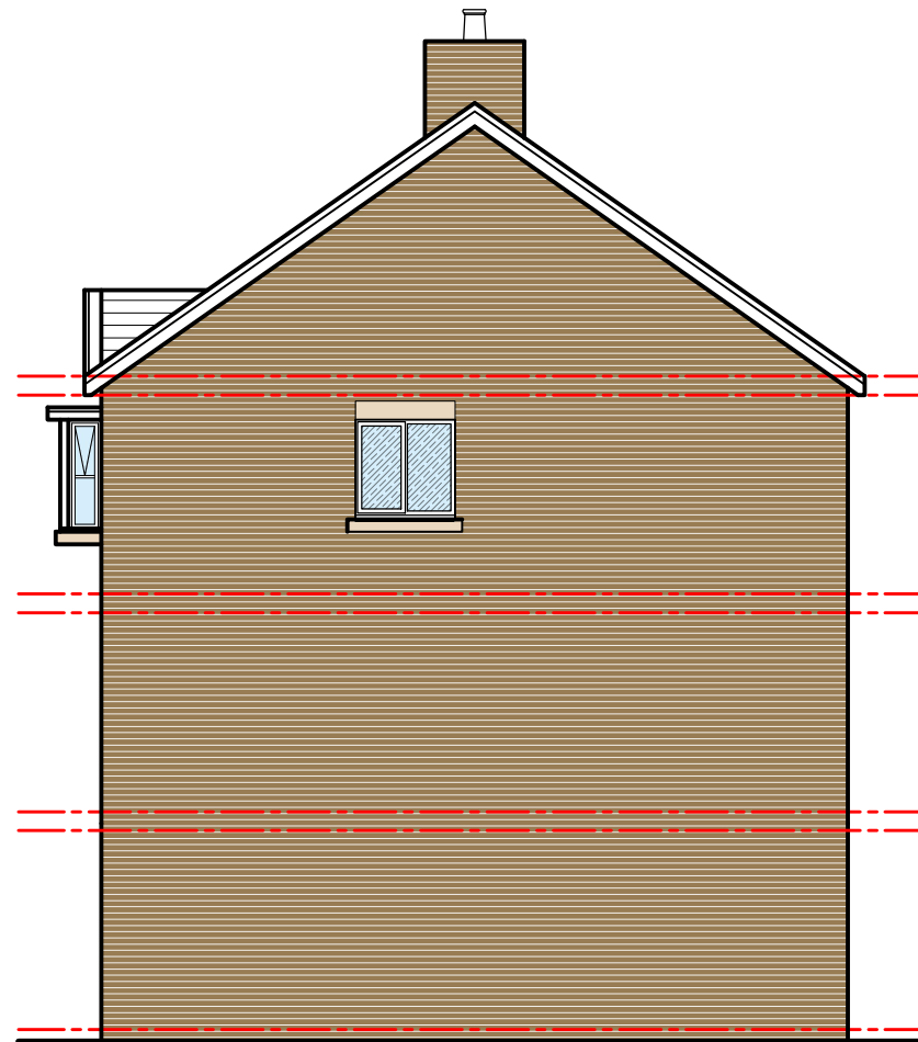
Side Elevation
