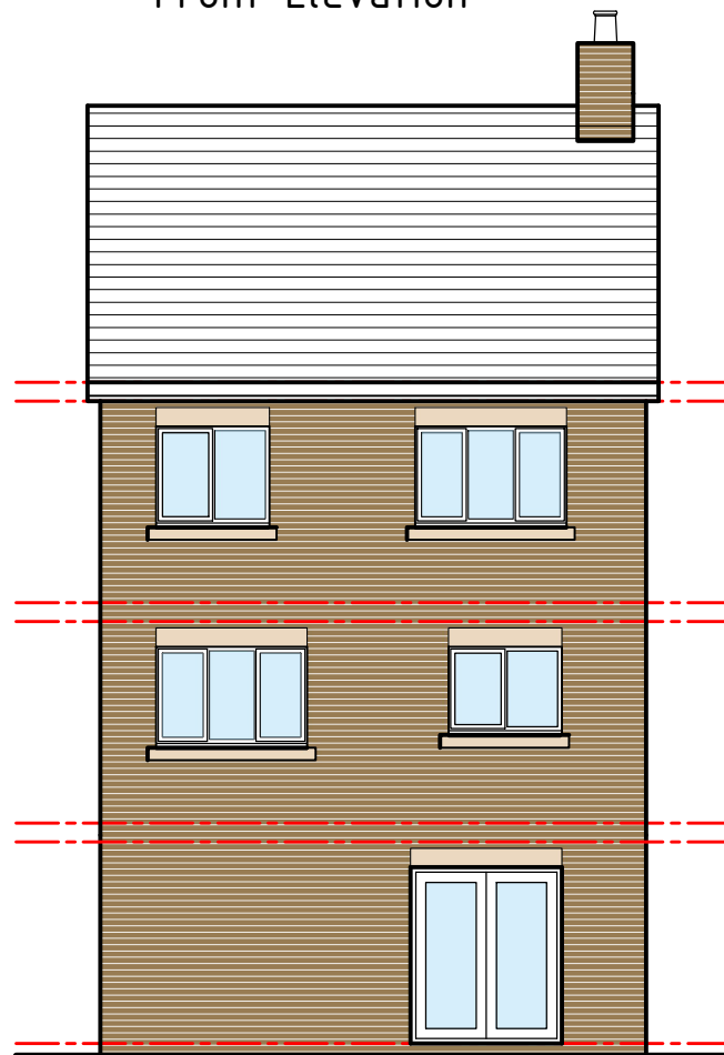
Rear Elevation
