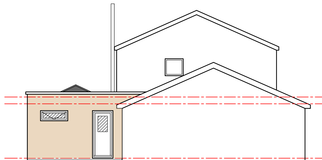
Side 02 Elevation
