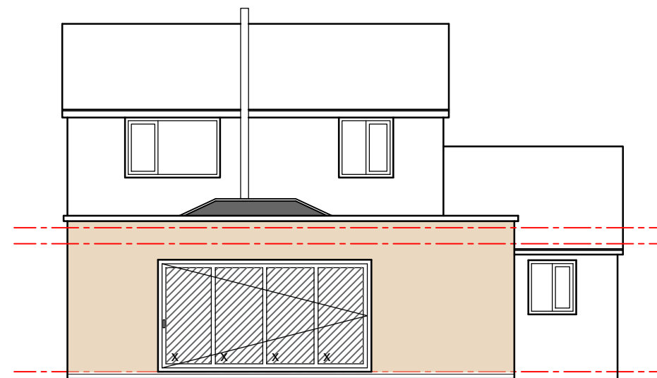
Rear Elevation
