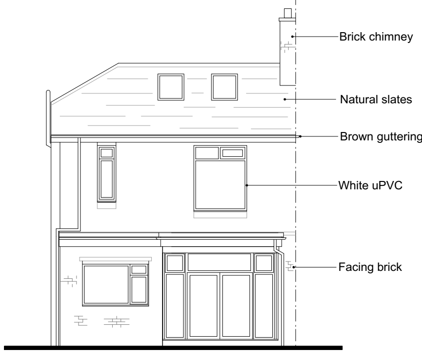
Existing Rear Elevation View C - 1:100
