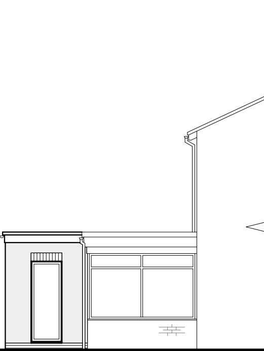
Proposed Side Elevation View D - 1:100
