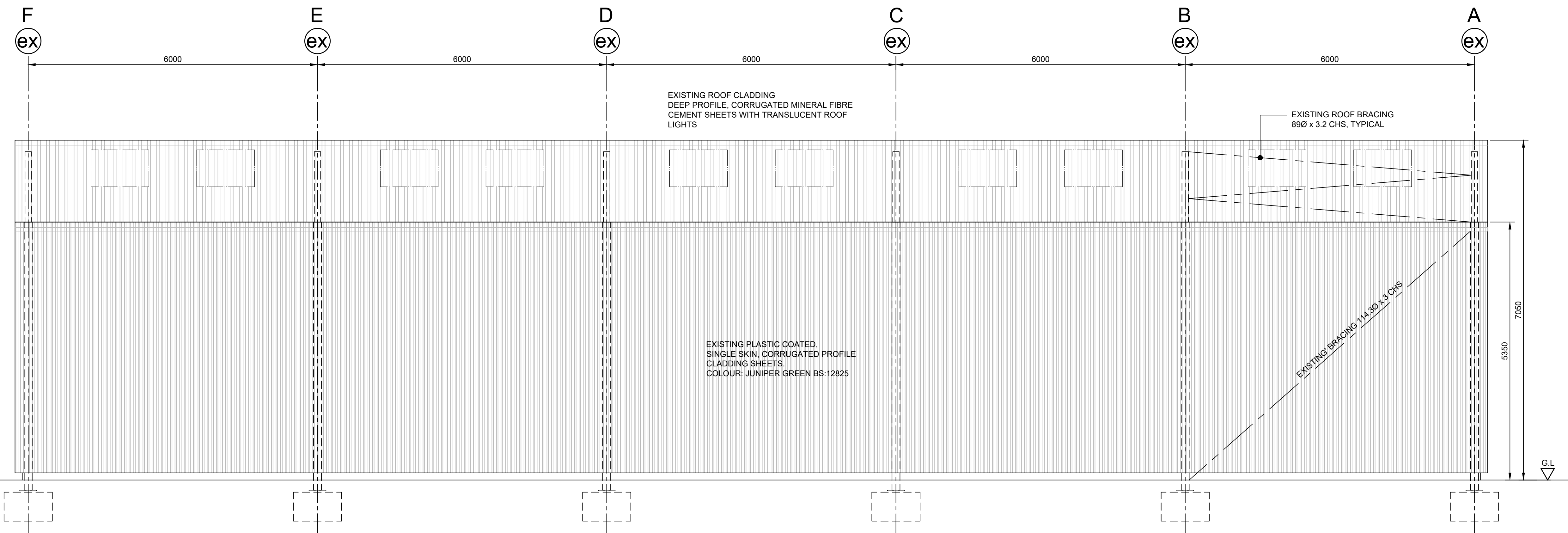
EXISTING ELEVATION ON GRID LINE 4
