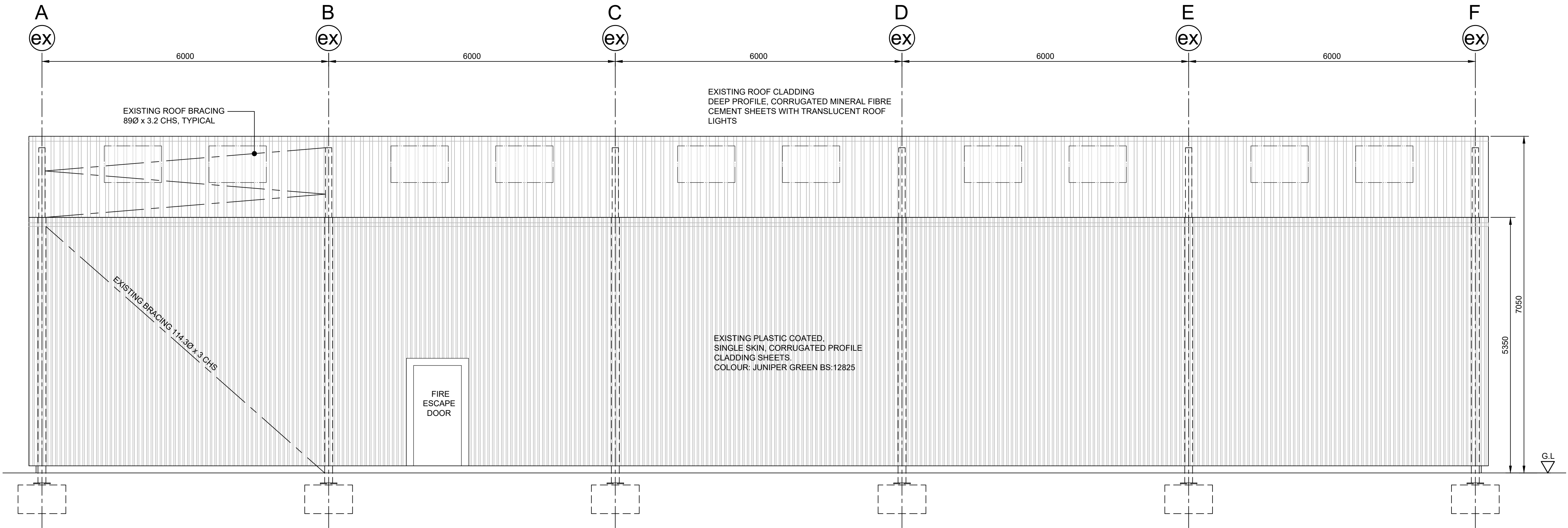
EXISTING ELEVATION ON GRID LINE 1
