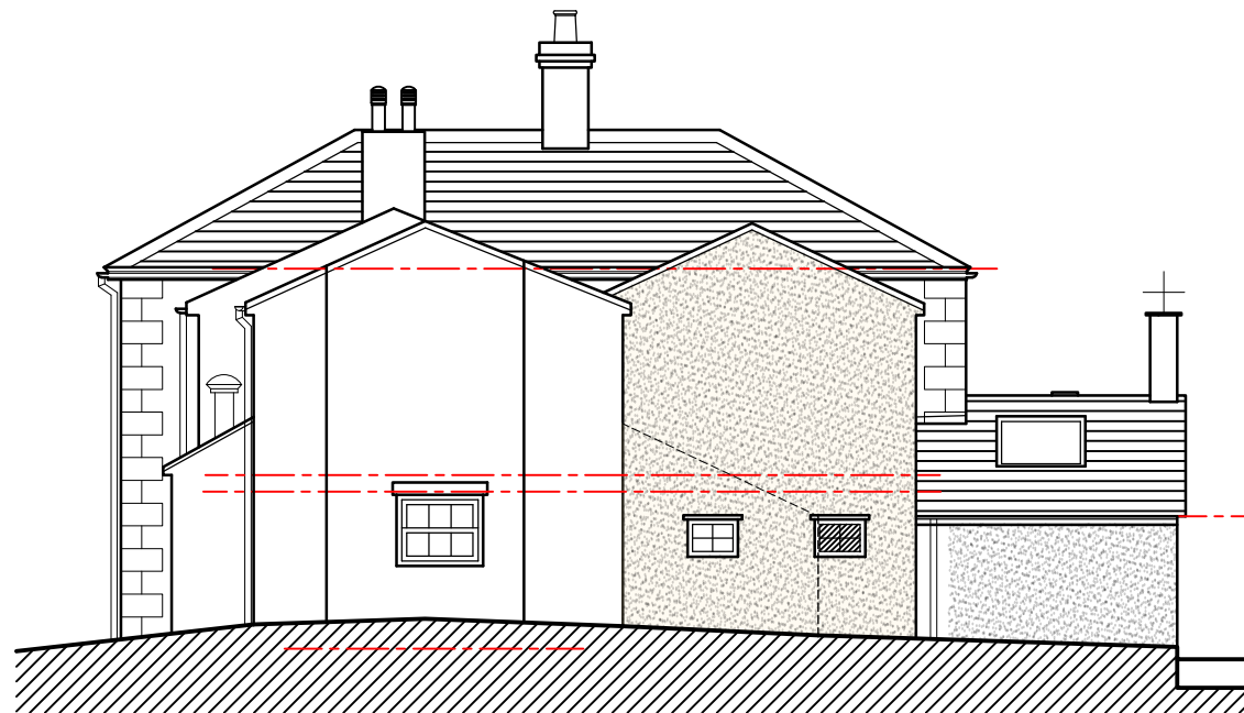
Rear Elevation
