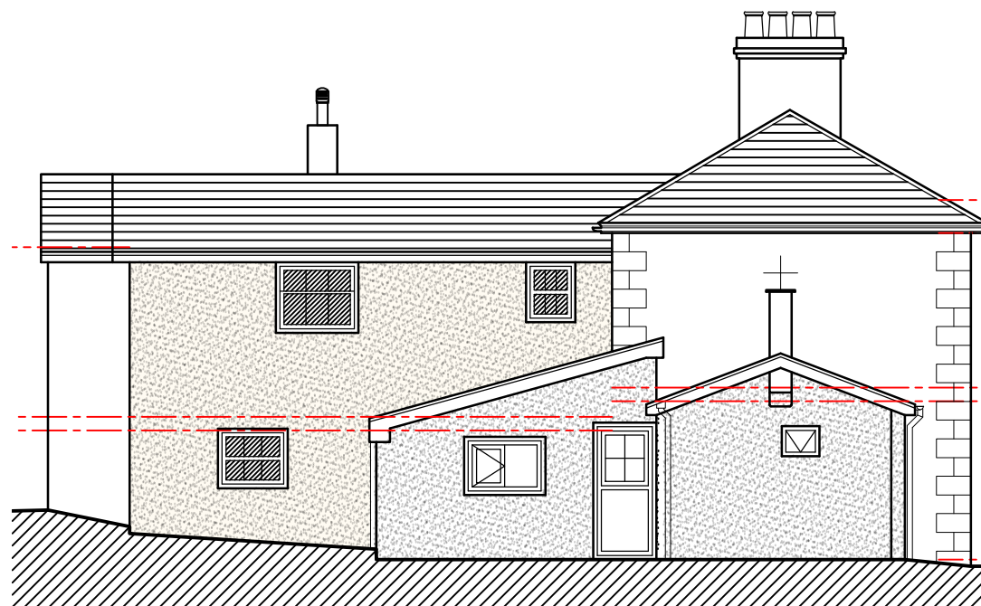
Side 02 Elevation
