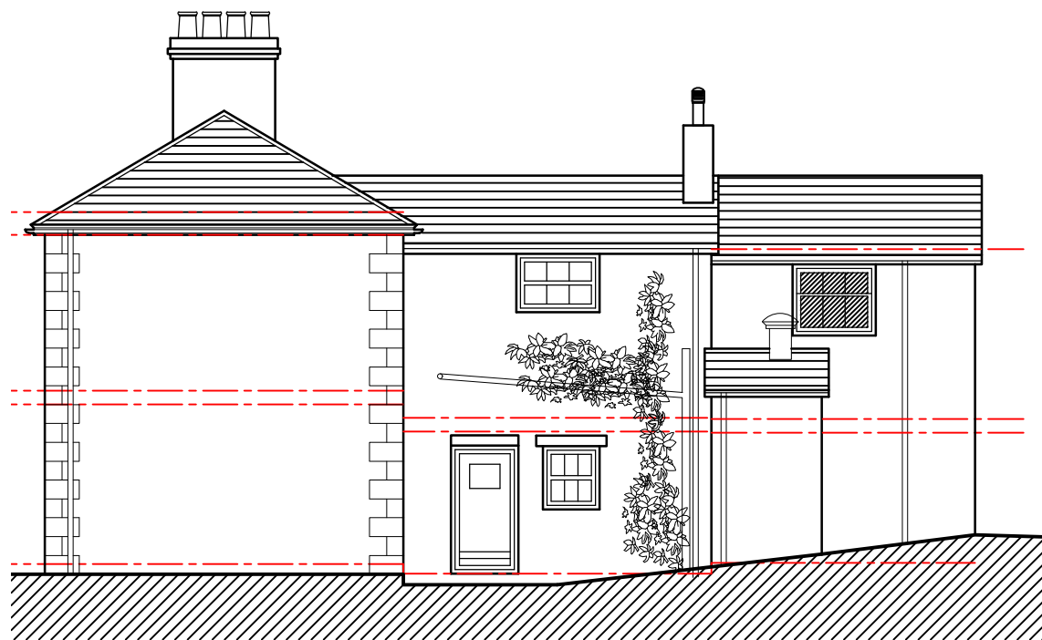
Side 01 Elevation
