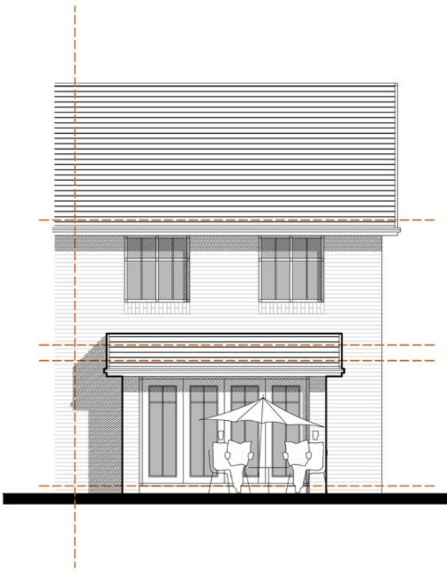
REAR ELEVATION
