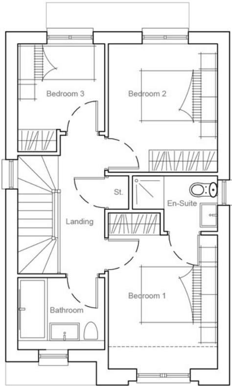
FIRST FLOOR 46 sqm
