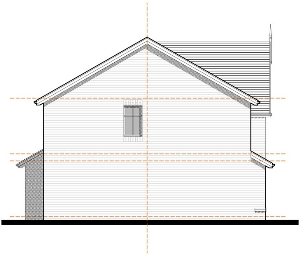
SIDE ELEVATION (LEFT)
