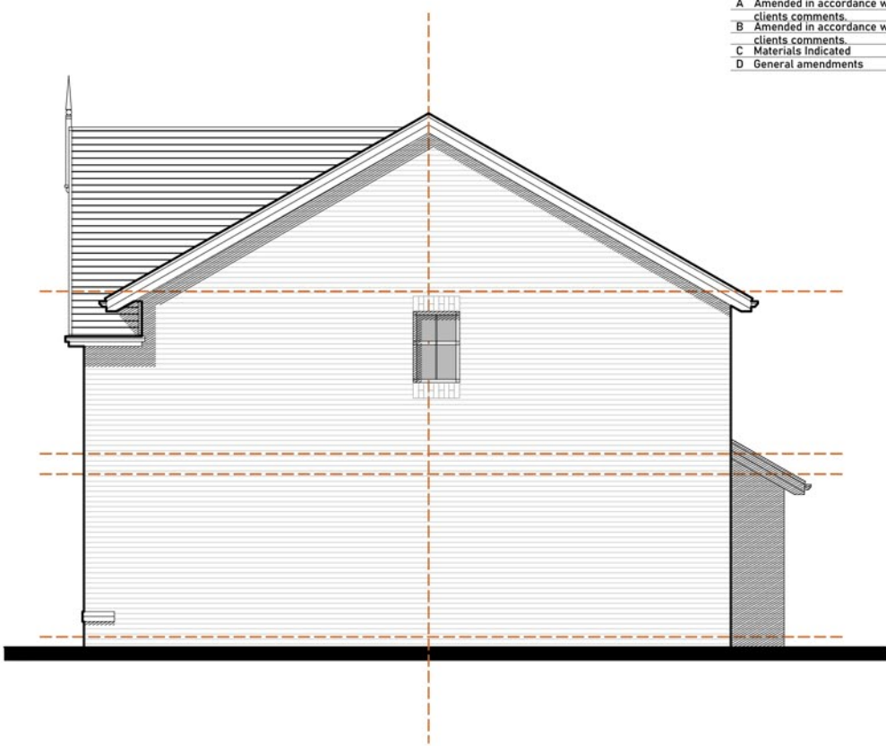
SIDE ELEVATION (RIGHT)
