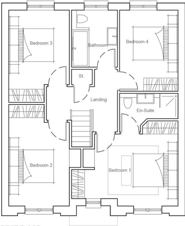
FIRST FLOOR 68.5 sqm
