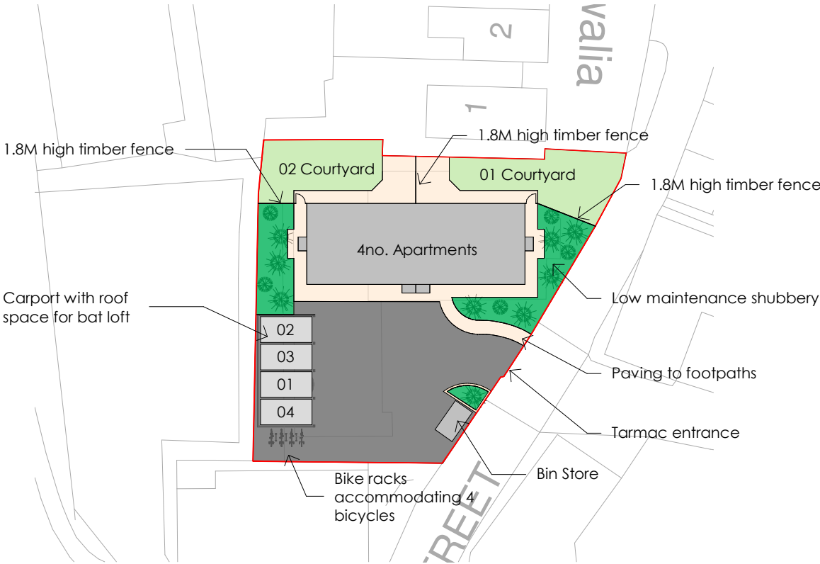
Proposed Site Plan 1 : 500
