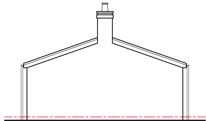
Side 02 Elevation
