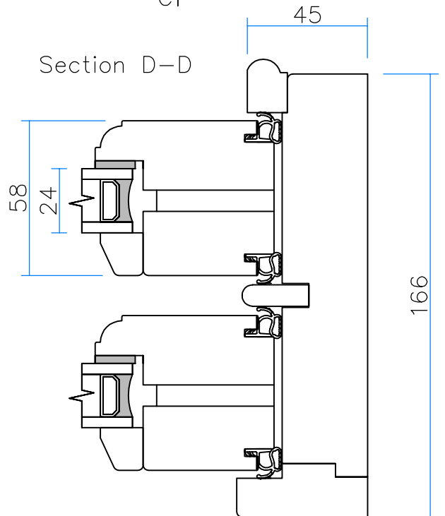
Georgain Bar Sections
