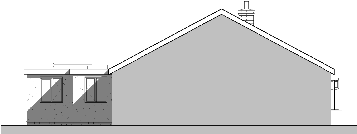
Side Elevation 2 1 : 100
