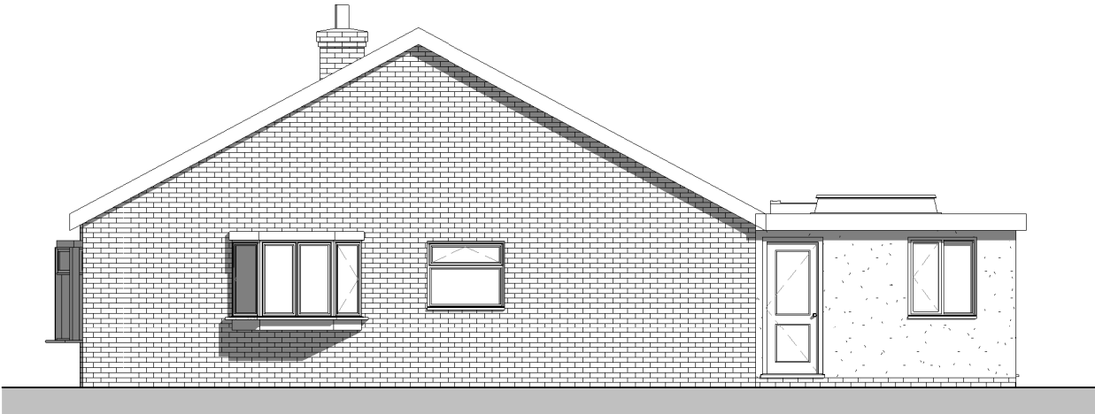
Side Elevation 1 1 : 100
