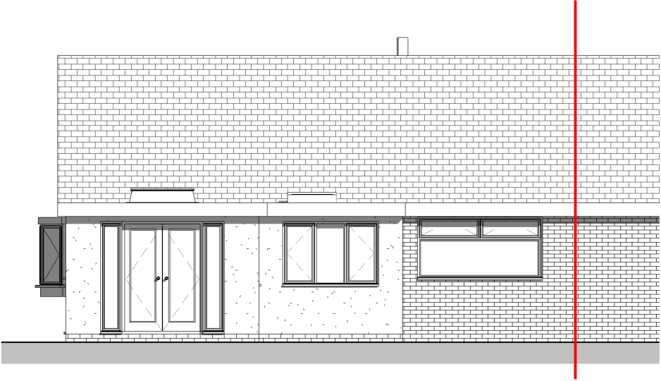
Rear Elevation 1 : 100
