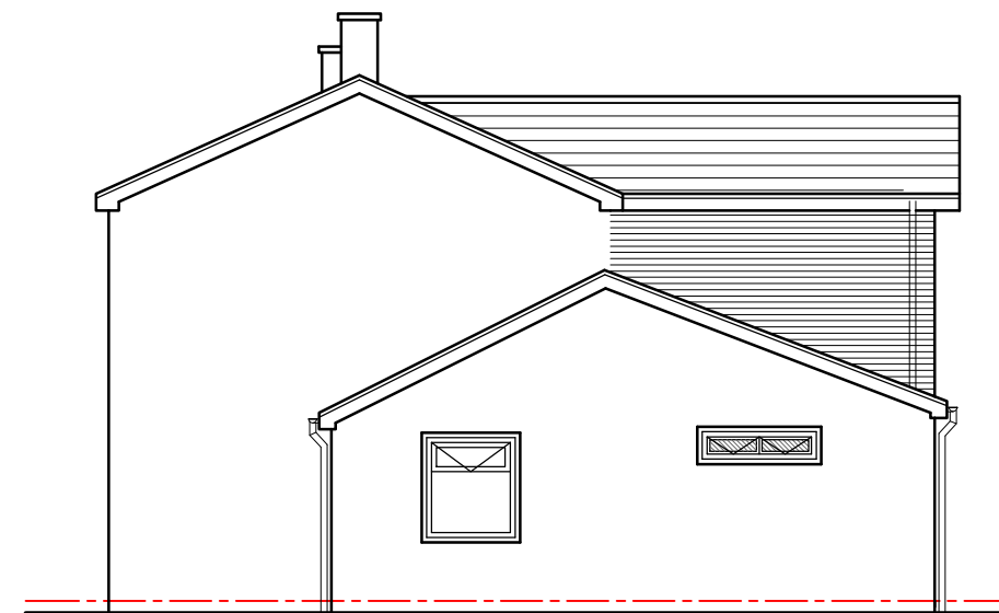
Rear Elevation
