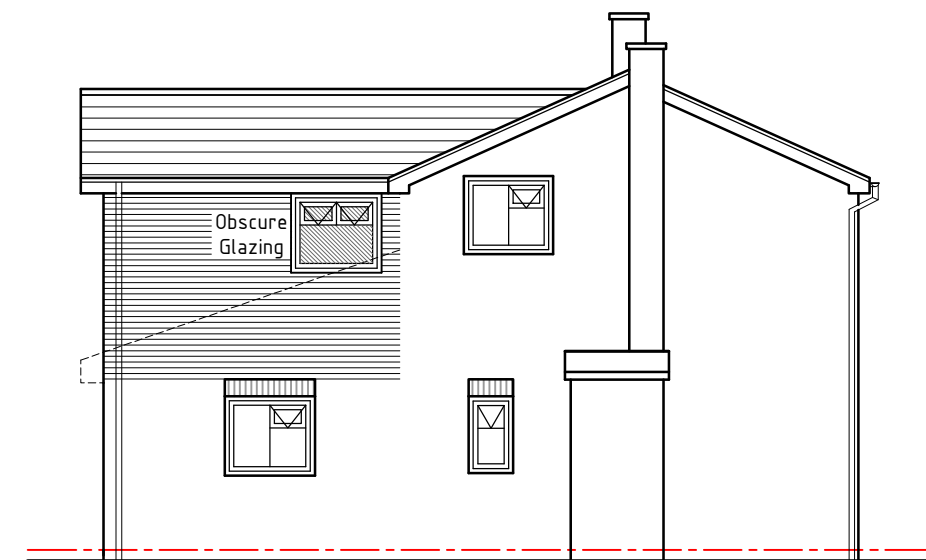
Side 01 Elevations
