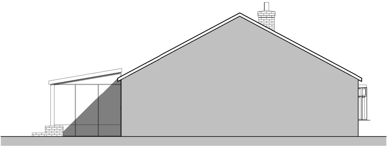
Side Elevation 2 1 : 100
