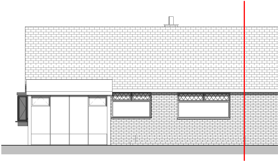
Rear Elevation 1 : 100
