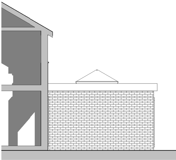
Side Elevation 1 : 100
