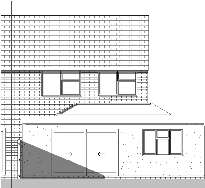
Rear Elevation 1 : 100
