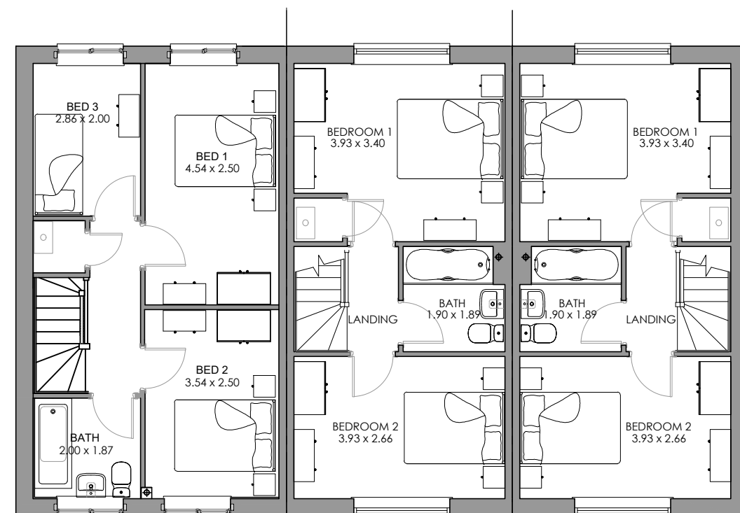
ELWY AS GROUND FLOOR CLWYD MID AS GROUND FLOOR CLWYD END OPP GROUND FLOOR
