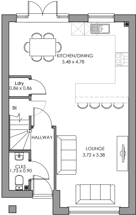
GROUND FLOOR OPEN PLAN
