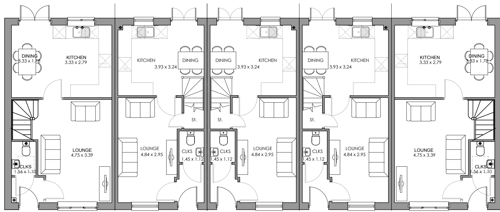
ELWY AS GROUND FLOOR
