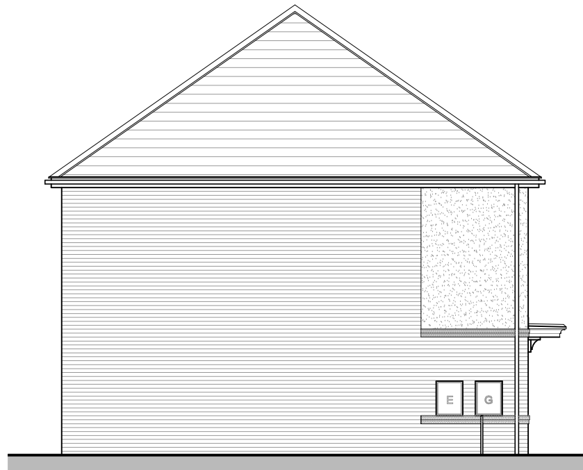
ELWY AS SIDE ELEVATION
