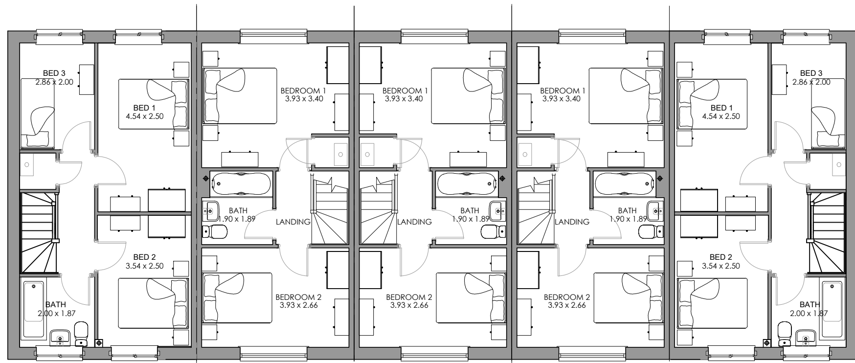
ELWY AS FIRST FLOOR
