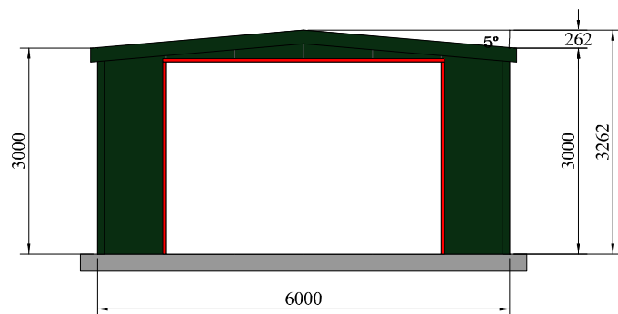
Front Elevation (External)
