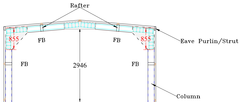
Cross Section (Scale = 1:75)
