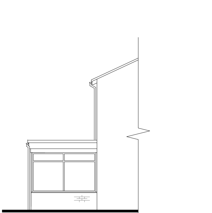
Existing Side Elevation View D - 1:100
