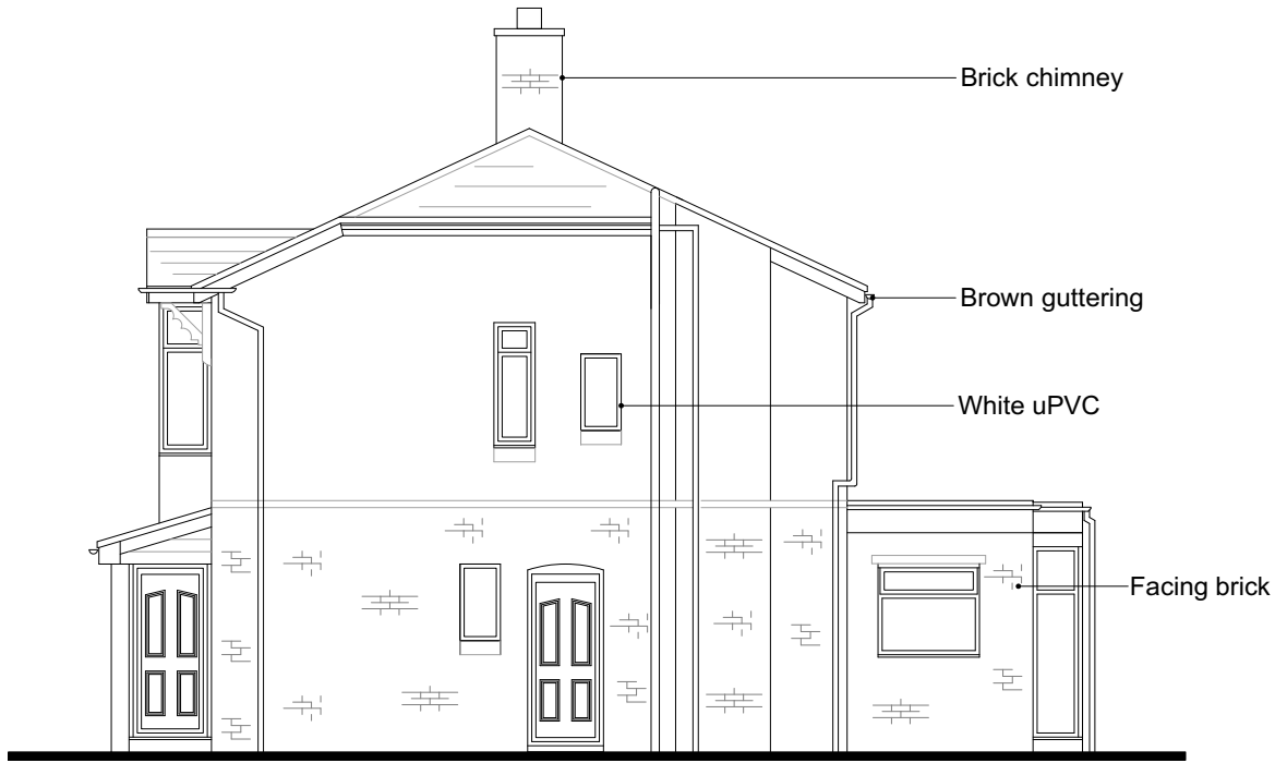
Existing Side Elevation View B - 1:100
