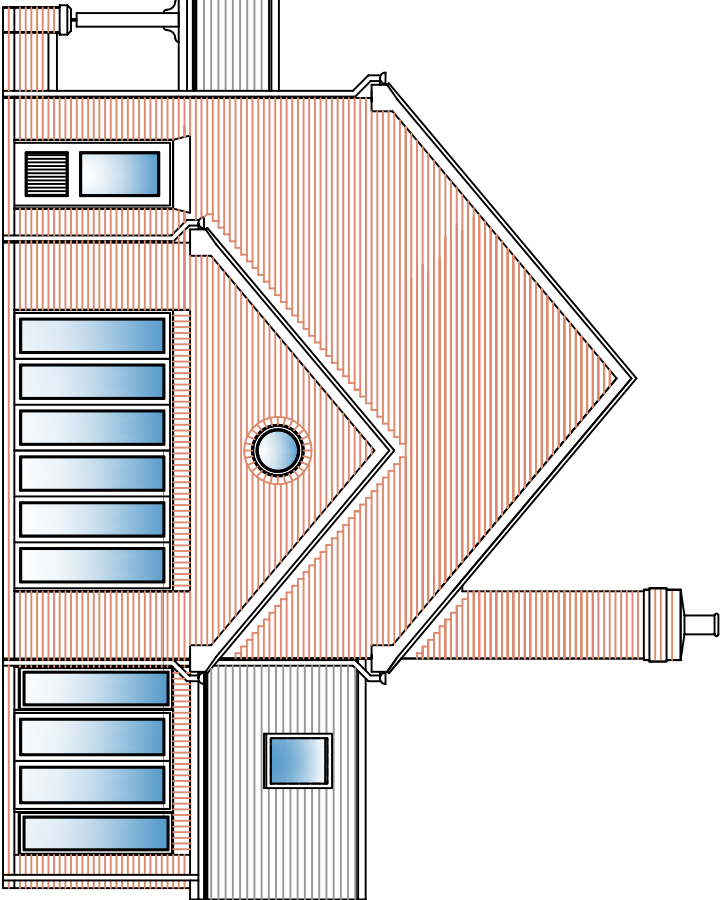
SOUTH (GARDEN) ELEVATION
