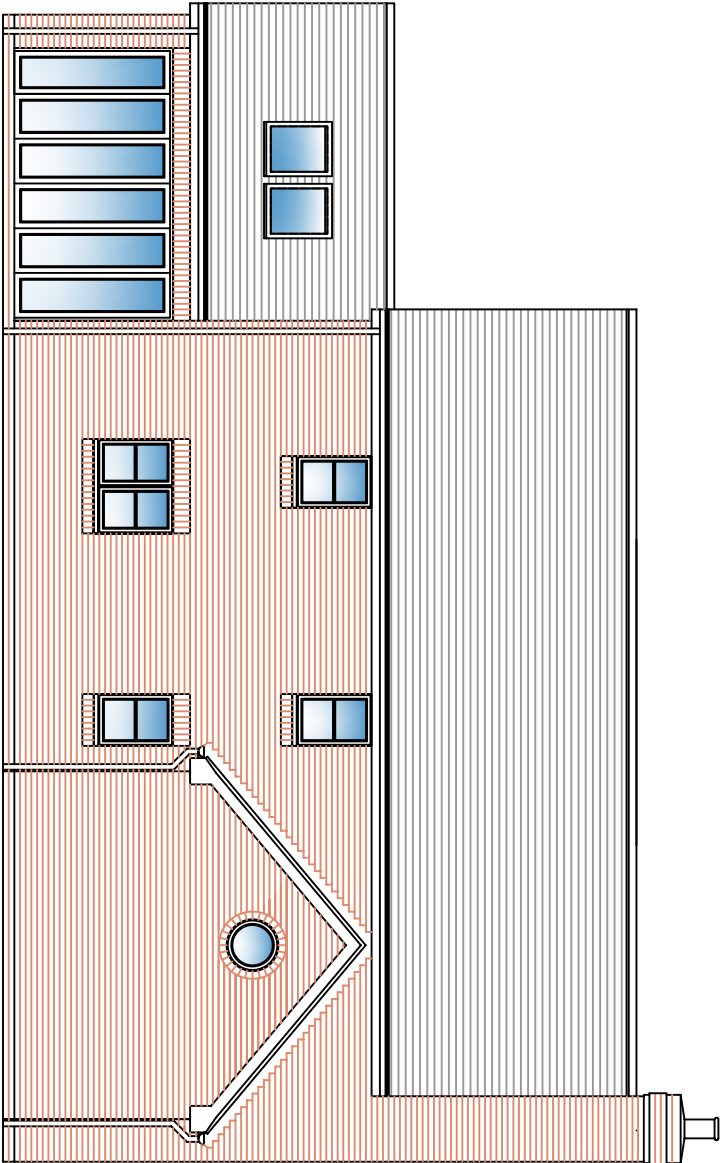
EAST (REAR) ELEVATION
