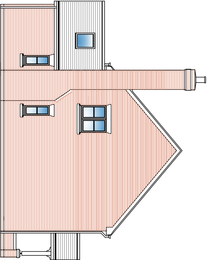
NORTH (GABLE) ELEVATION
