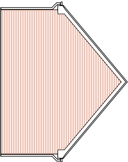
GABLE ELEVATION
