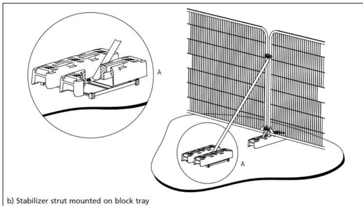
Tree Protective Fencing Specification
