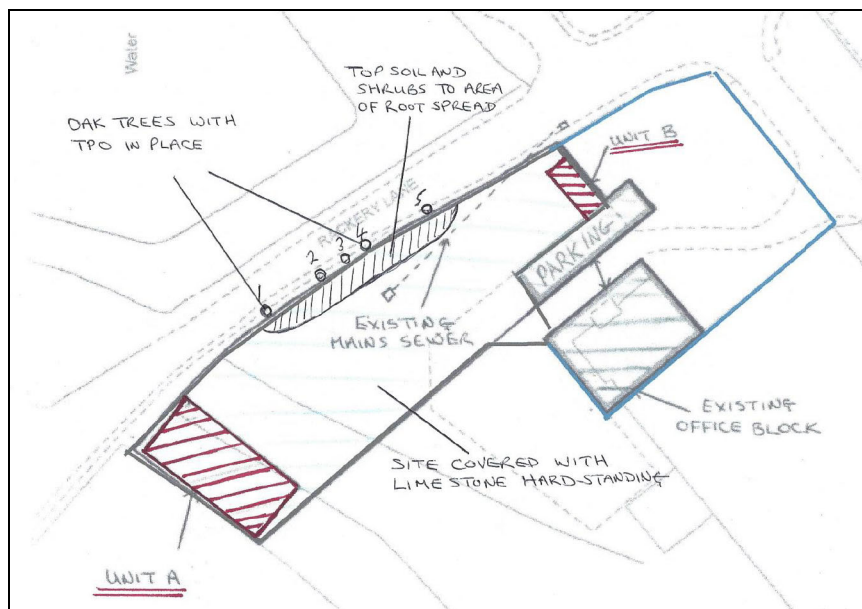
Plate 1 – Previous layout with Unit B & hard standing within RPA of trees
