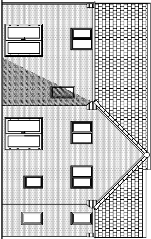
PROPOSED REAR ELEVATION
