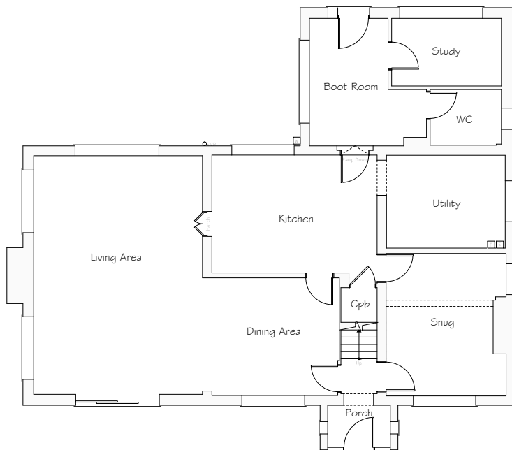
Ground Floorplan 1:50
