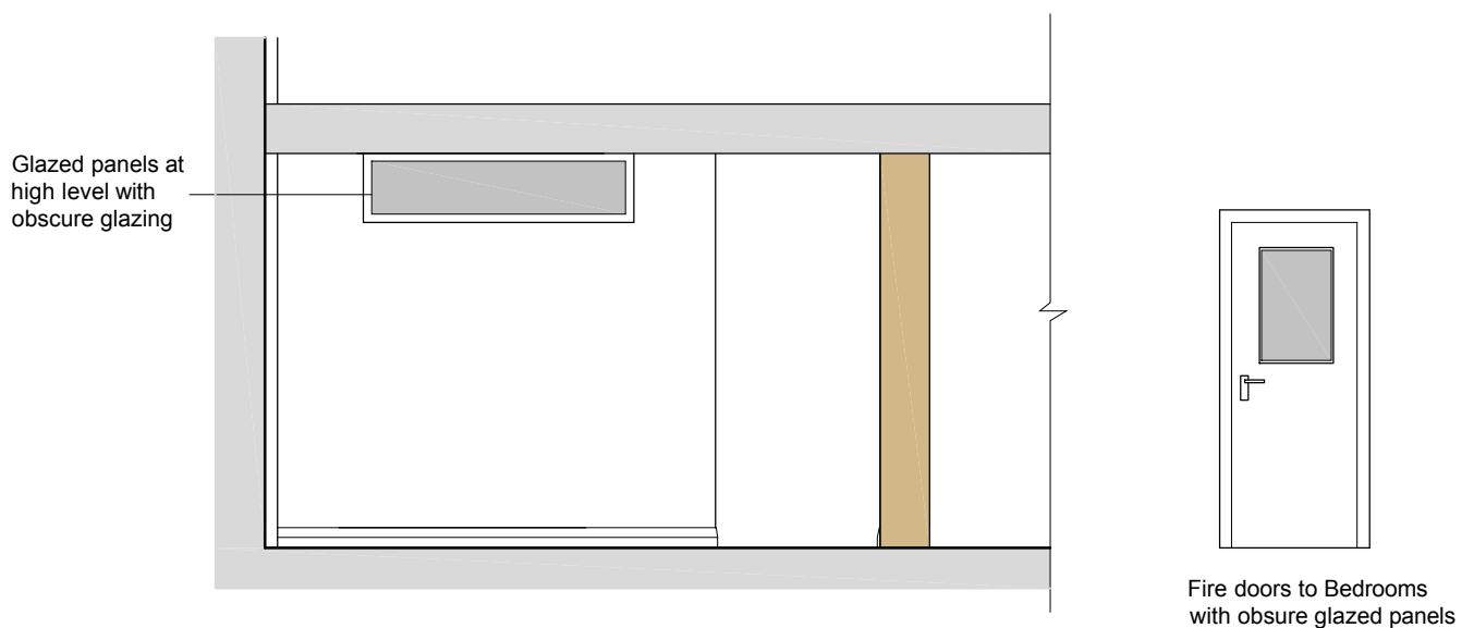
FLAT 3 - Glazed screen
