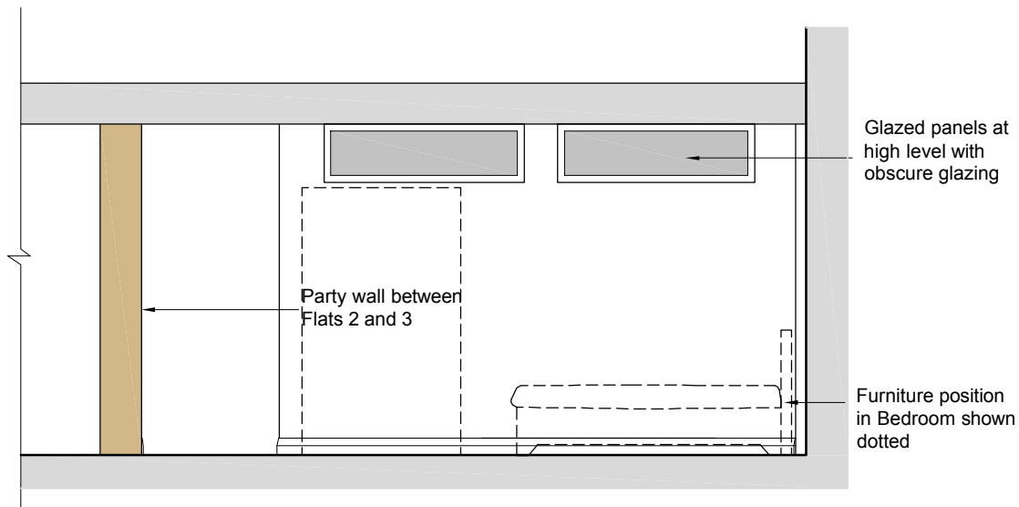
FLAT 2 - Glazed screen
