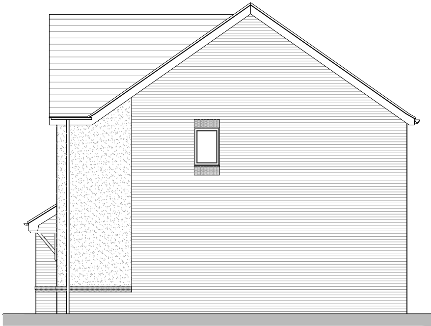
SIDE ELEVATION
