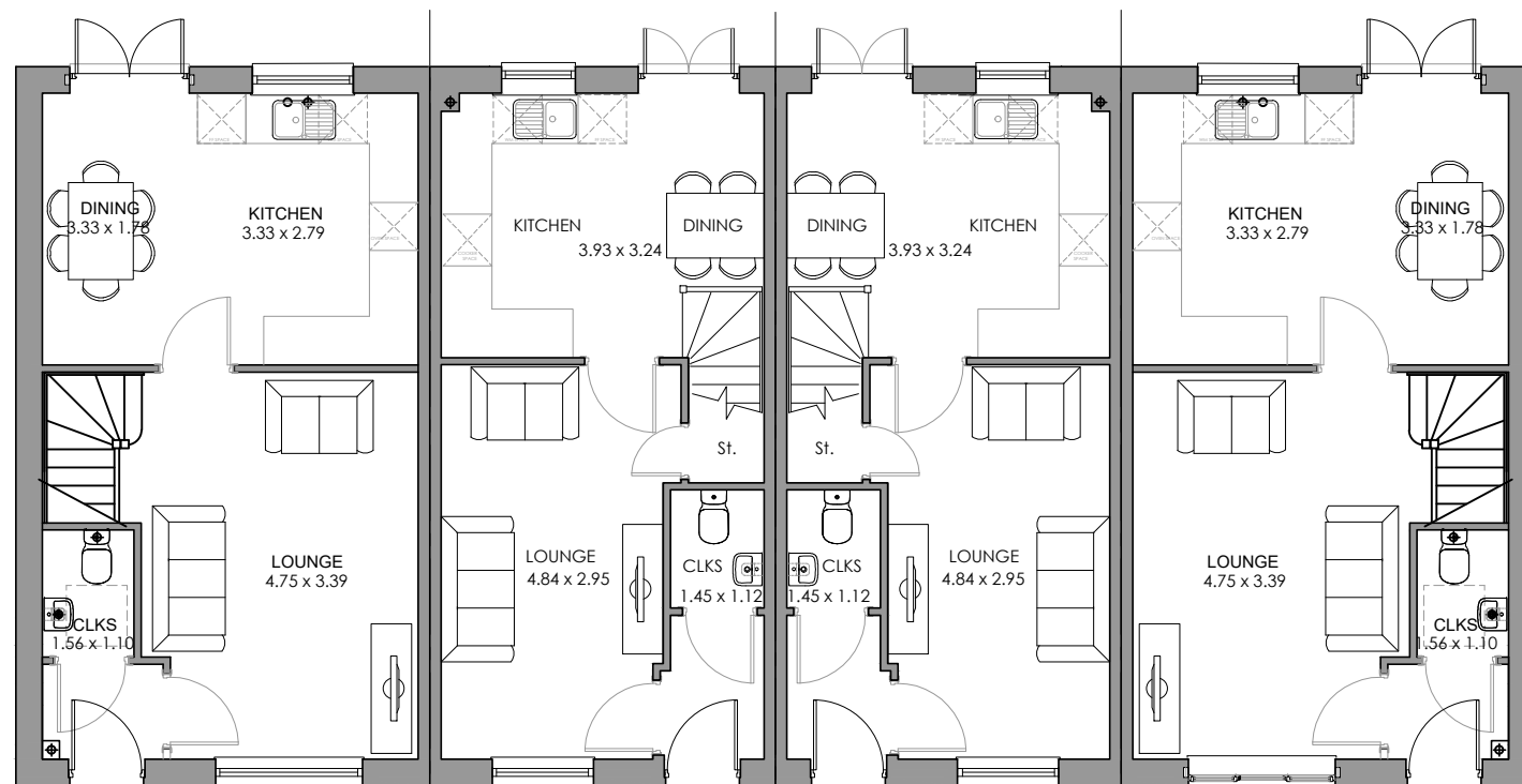
HIGHFIELD AS GROUND FLOOR
