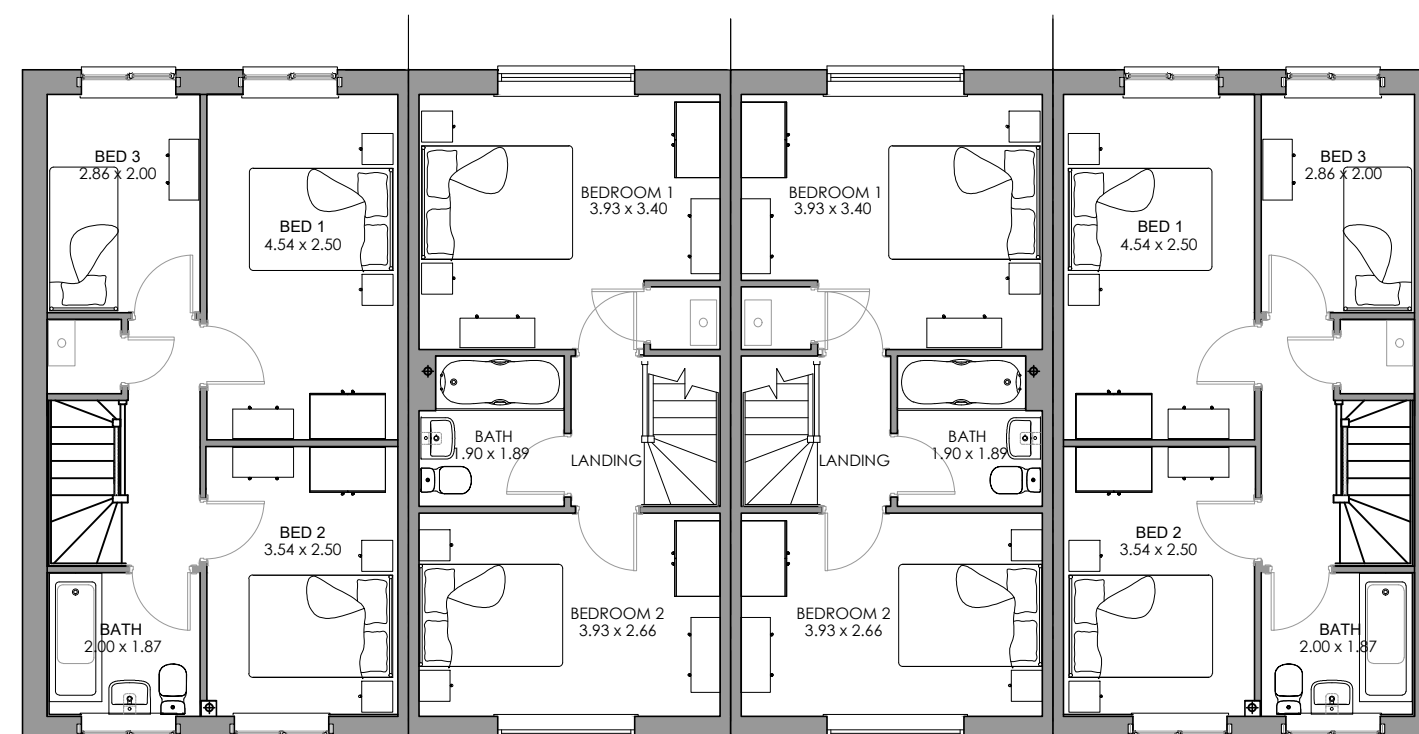
HIGHFIELD AS FIRST FLOOR
