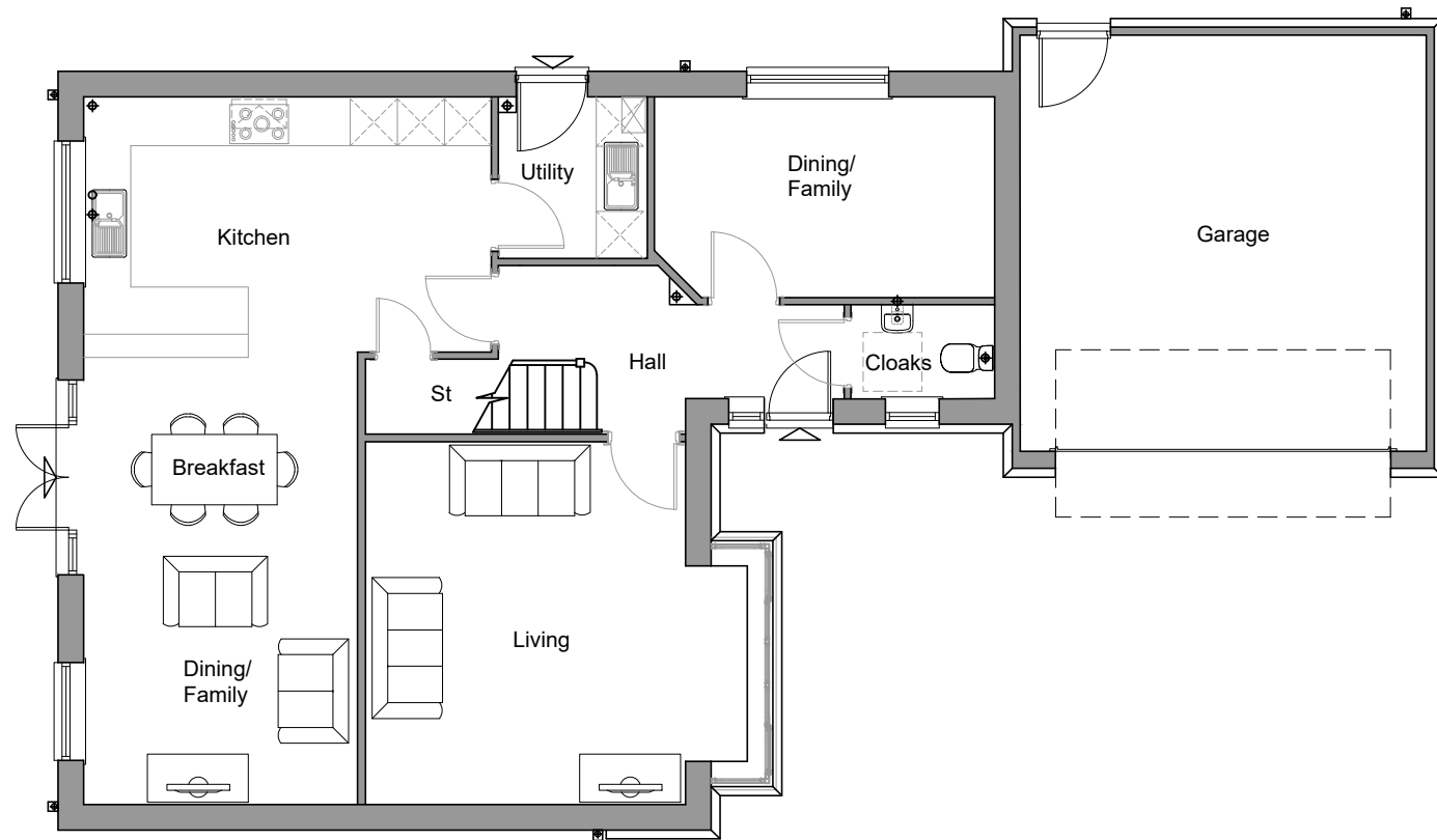
GROUND FLOOR
