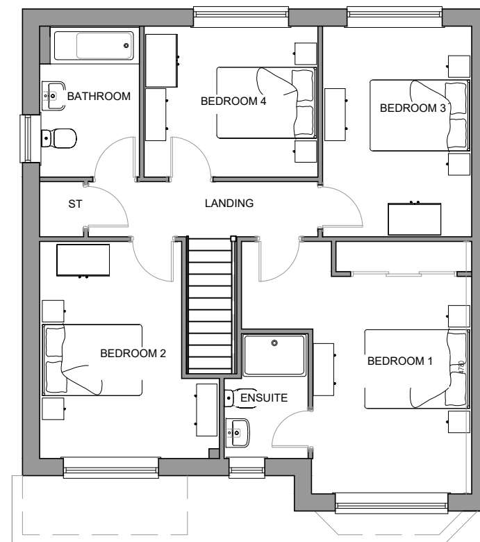
FIRST FLOOR
