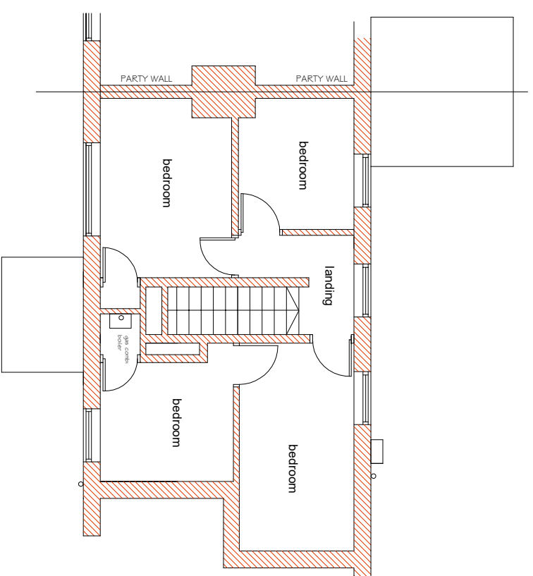
EXISTING FIRST FLOOR PLAN SCALE 1:50
