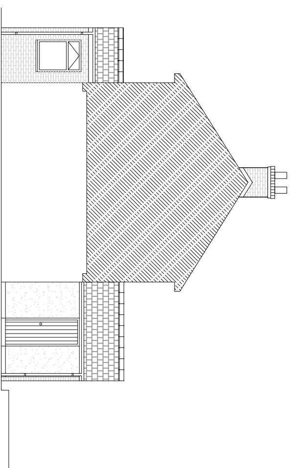
Existing Side Elevation. scale 1:50
