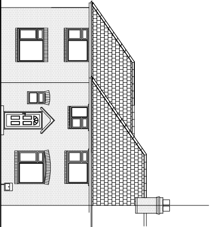
PROPOSED FRONT ELEVATION
