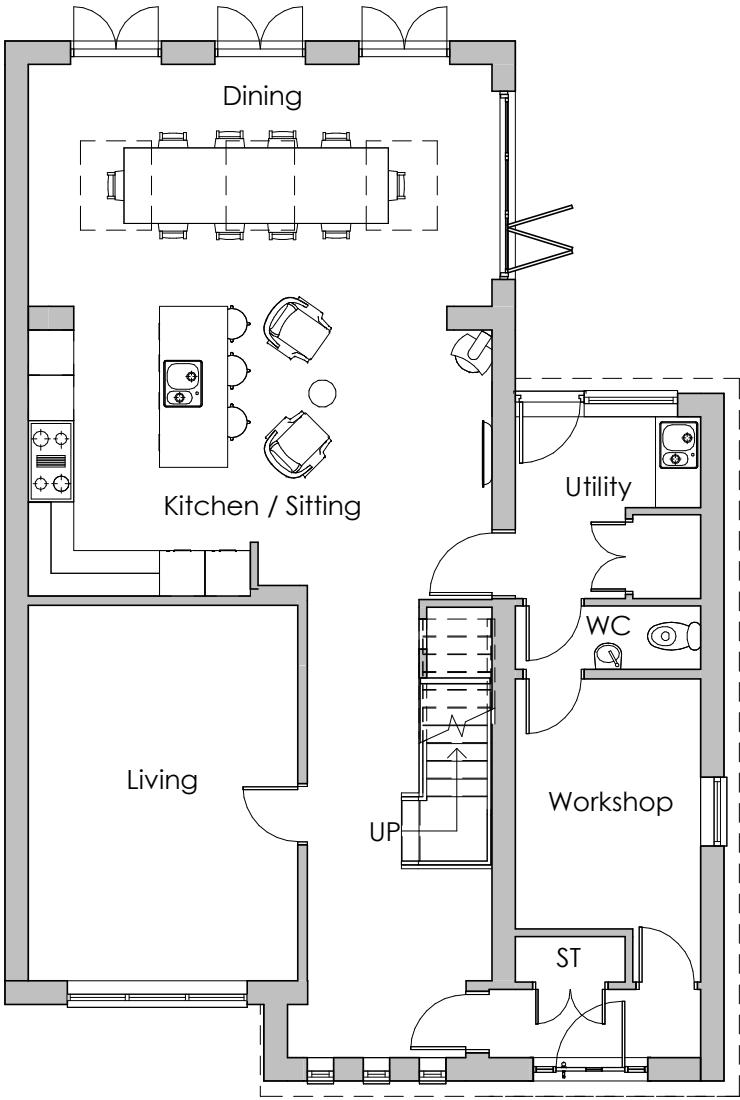
Ground Floor 1 : 100
