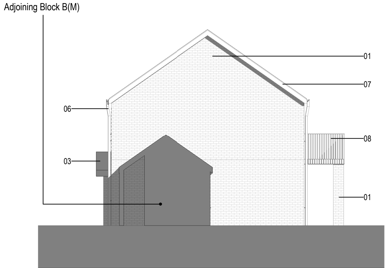
Side Elevation 1 : 100
