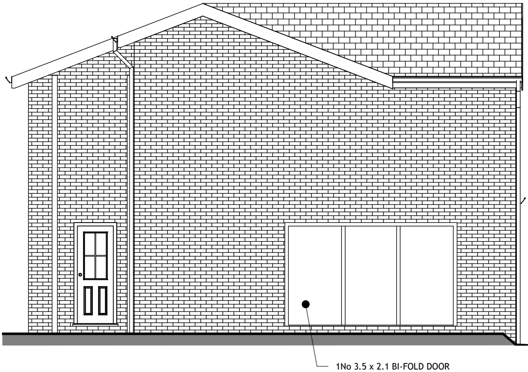
2 PLANNING AMENDMENT TO SE ELEVATION 1 : 75
