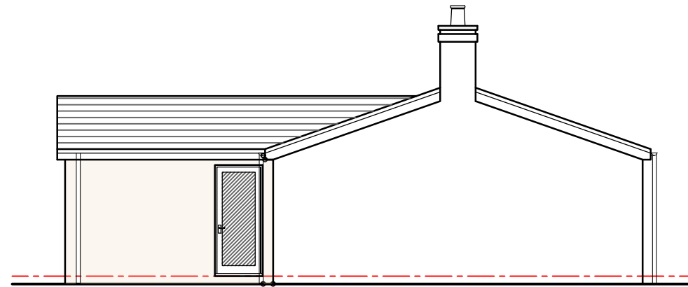
Side 02 Elevation
