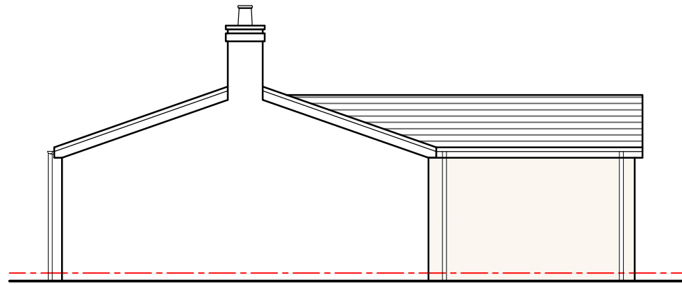
Side 01 Elevation
