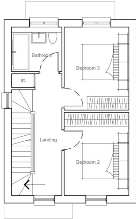
FIRST FLOOR 37.5 sqm
