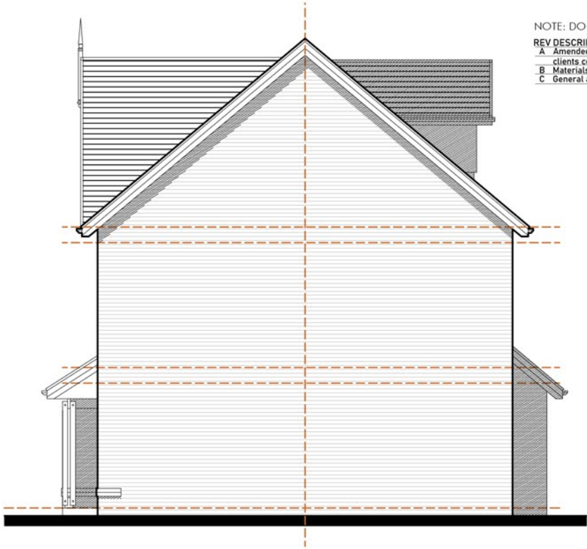
SIDE ELEVATION (RIGHT)
