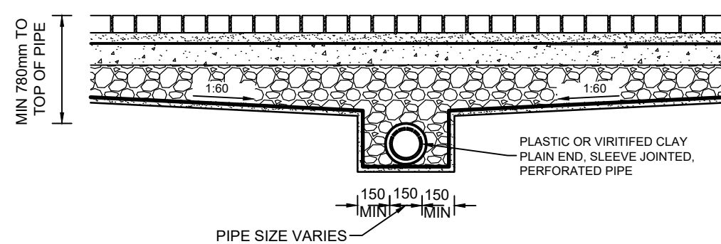
TYPICAL TYPE C POROUS PAVING CONSTRUCTION 1:25
