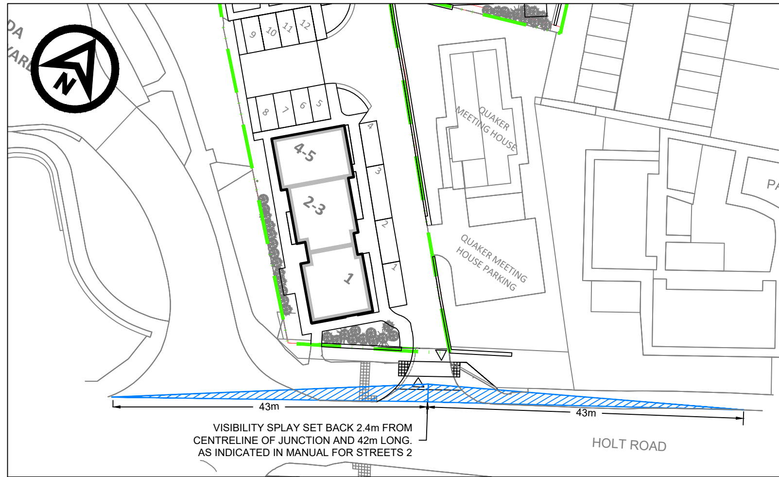
VISIBILITY SPLAY 1:500
