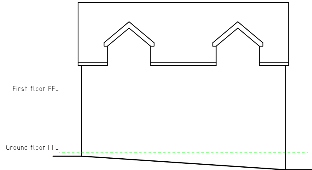
Front Elevation
