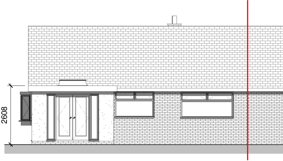
Rear Elevation 1 : 100
