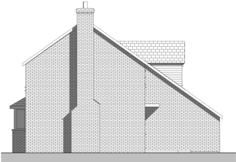
Side Elevation 1 : 100
