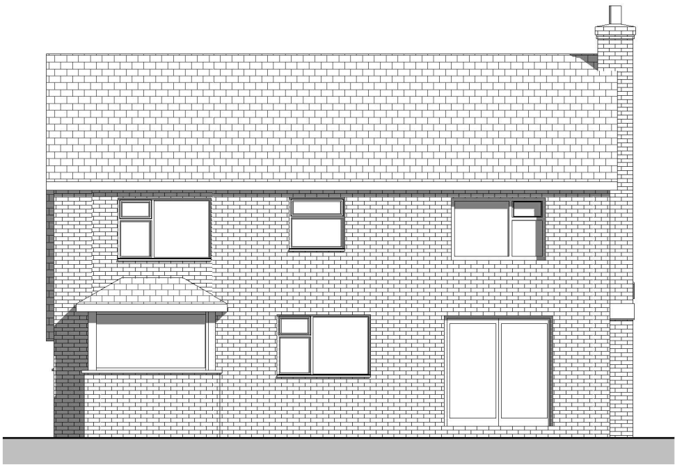
Rear Elevation 1 : 100
