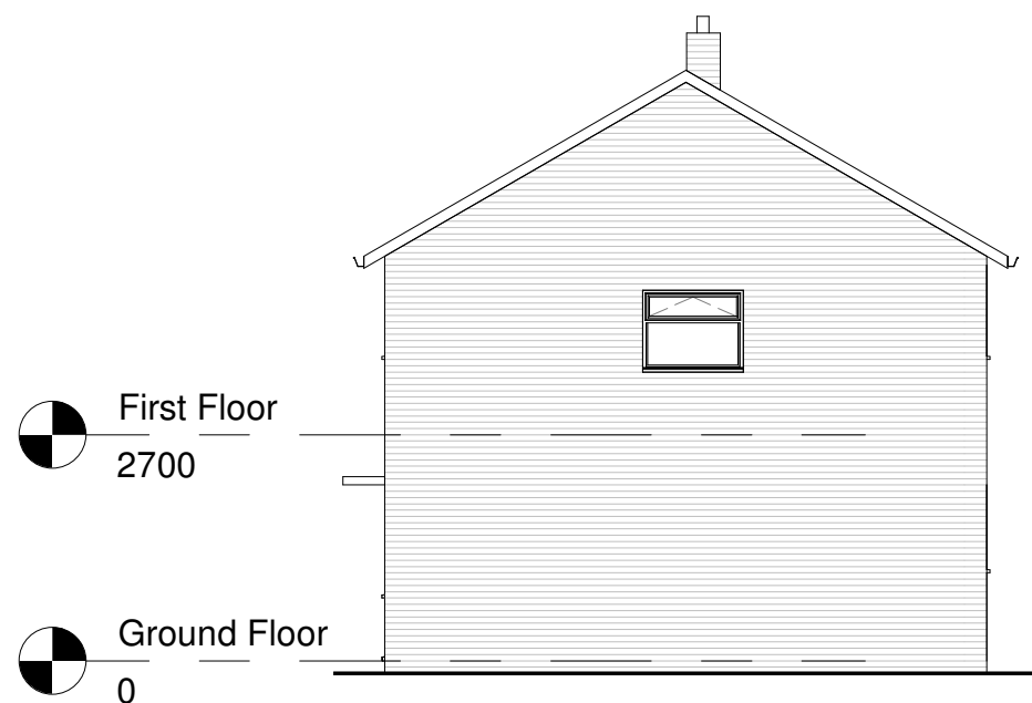
Existing North Elevation 1 : 100
