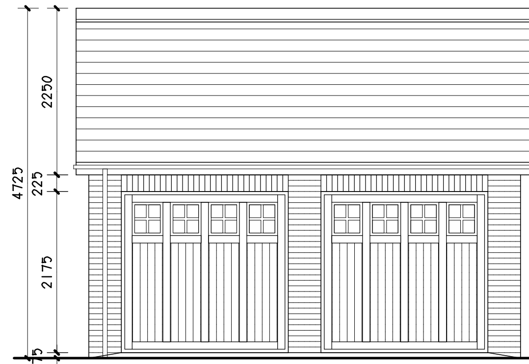
FRONT ELEVATION.
