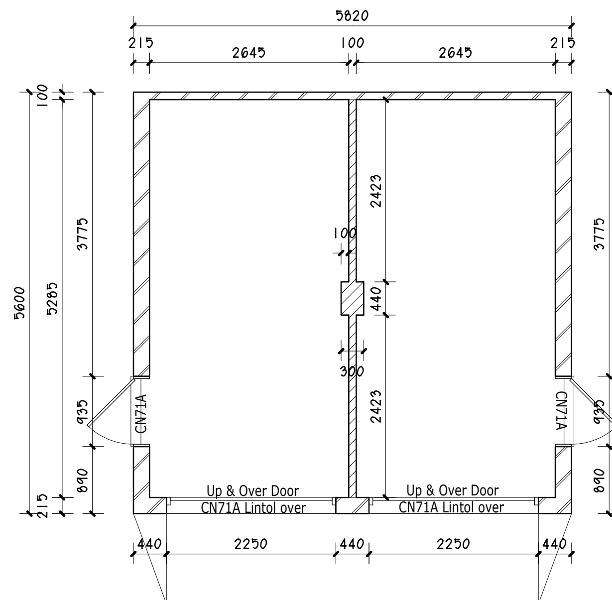
DOUBLE DETACHED GARAGE - PROPOSED FLOOR PLAN.
