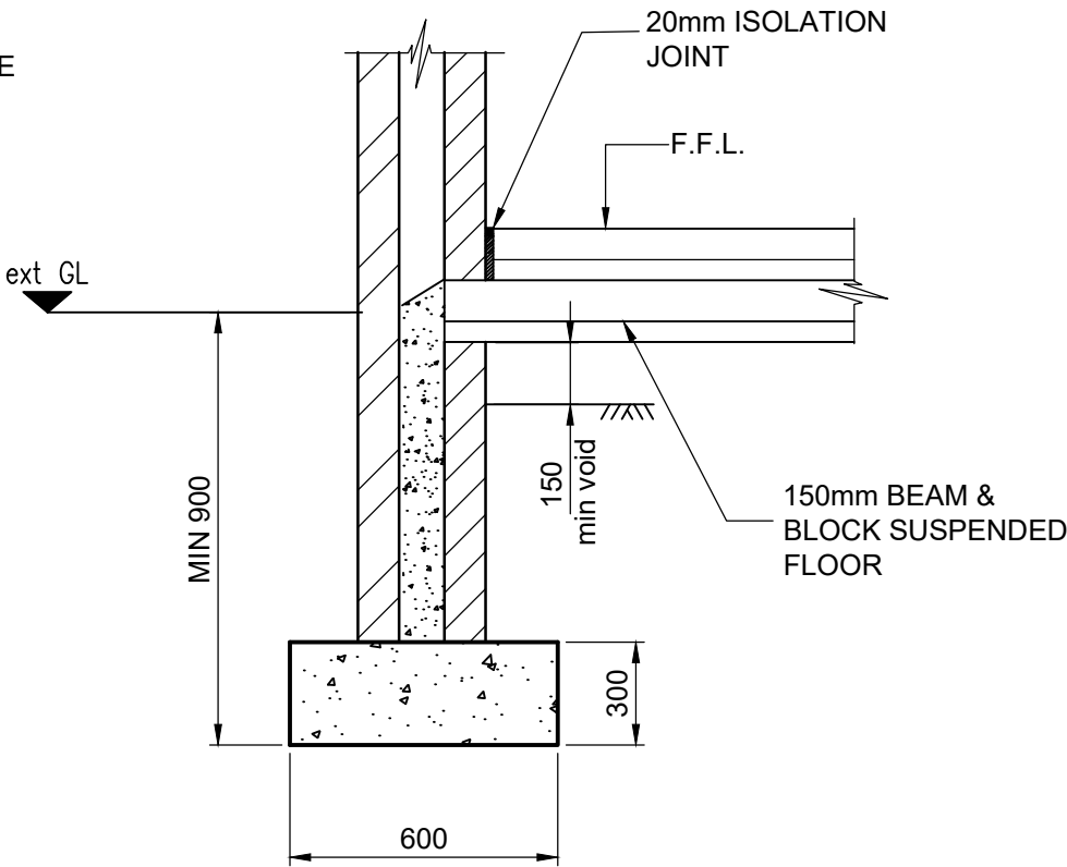
SECTION THROUGH REAR WALL
