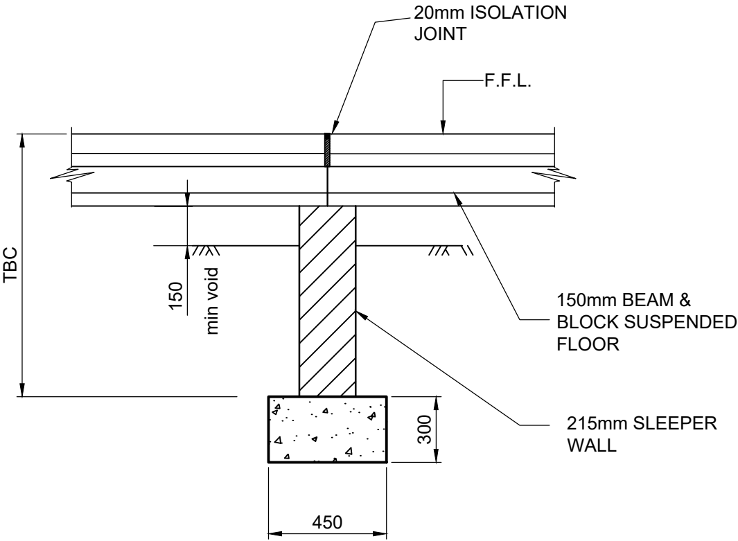
SECTION THROUGH SLEEPER WALL
