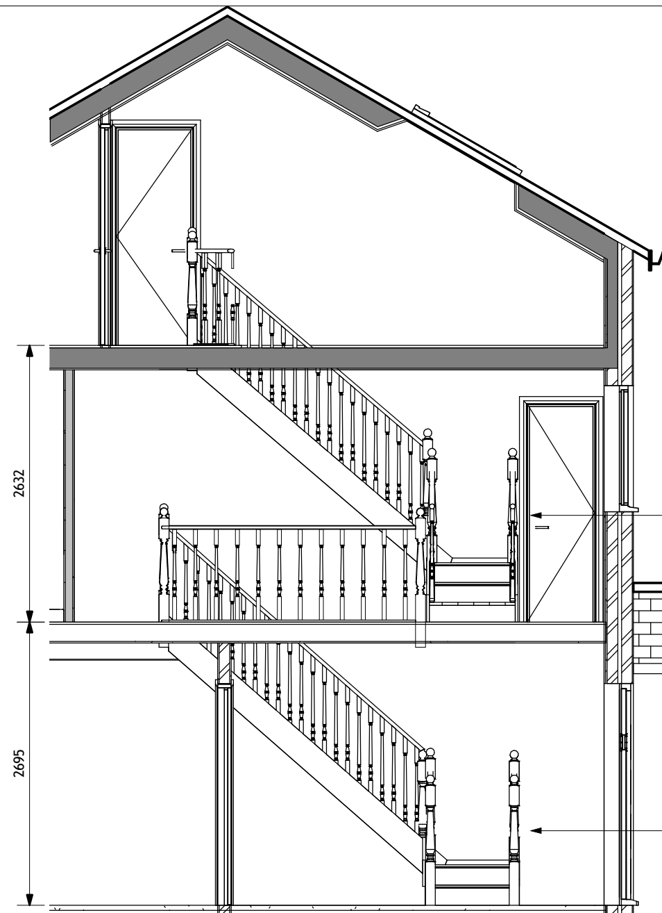
1 STAIRCASE ELEVATION 1 : 50
