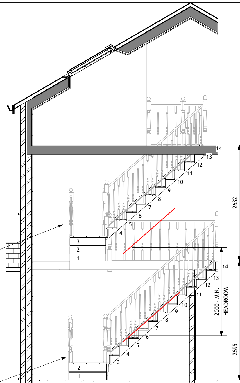
2 STAIRCASE SECTION 1 : 50
