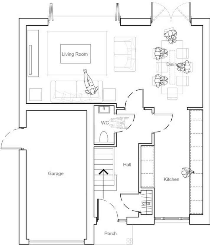
GROUND FLOOR TYPE B 52 sqm
