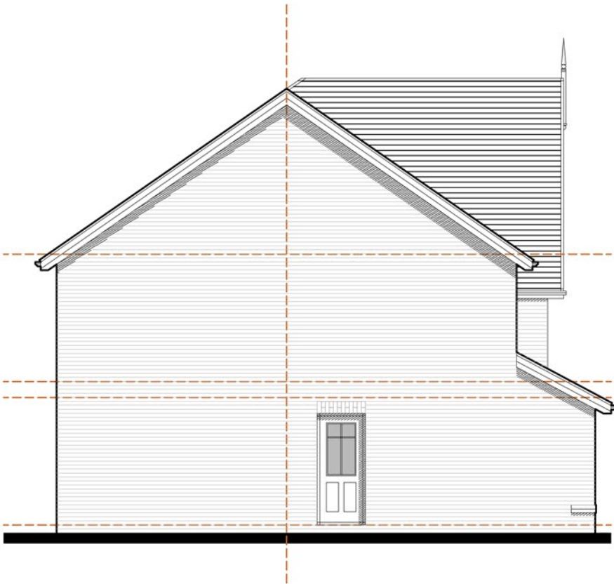
SIDE ELEVATION (LEFT)
