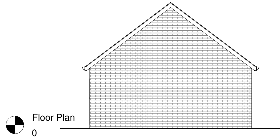
East Elevation 1 : 100
