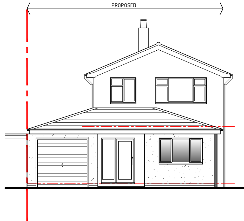
Front Elevation 1:100
