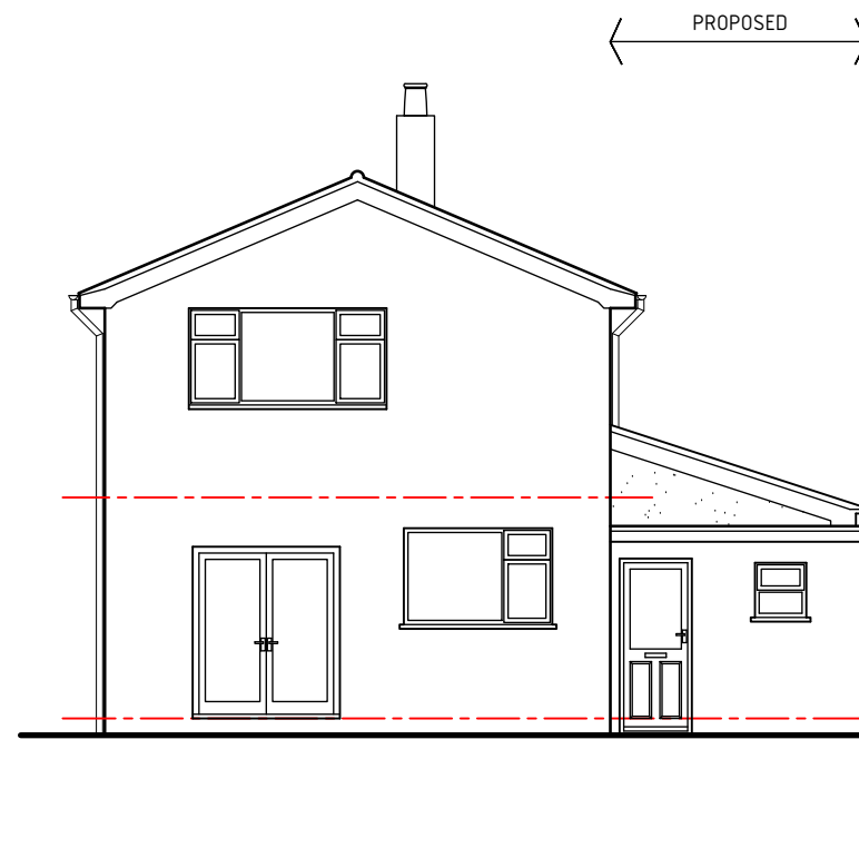
Rear Elevation 1:100
